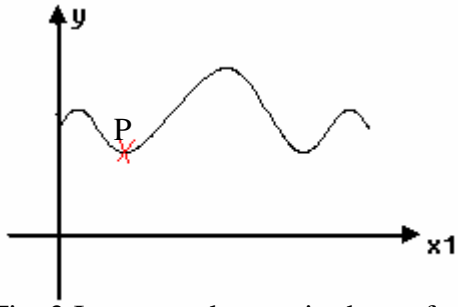
Fig. 3 Intercepted curve in the surface
