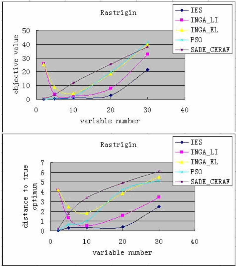
Fig. 14 Superiority of IES on Rastrigin problem (Problem 2)
