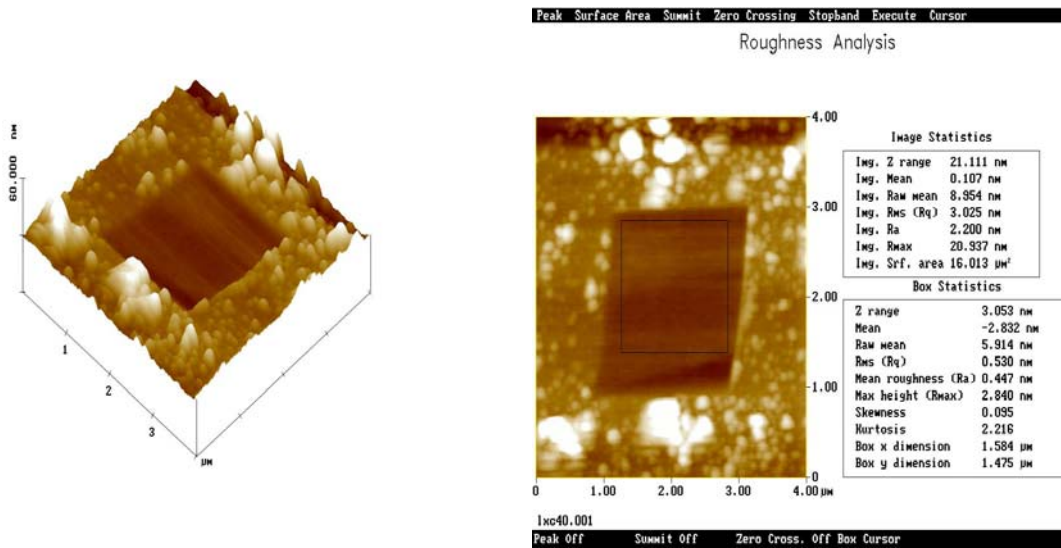
Fig. 8 Machined surface topography.
