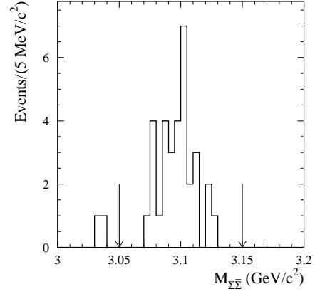
FIG. 24: The \Sigma^0 \bar{\Sigma}^0 mass spectrum for the mass region near the J/\psi . The arrows indicate the boundaries between the signal region and sideband regions.
