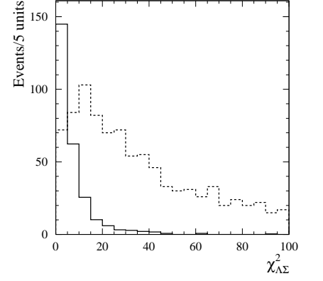
FIG. 20: The \chi^2_{\Lambda\Sigma} distributions for simulated events for e^+e^- \rightarrow \Lambda\bar{\Sigma}^0\gamma (solid histogram) and e^+e^- \rightarrow \Sigma^0\bar{\Sigma}^0\gamma (dashed histogram).
