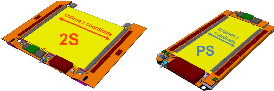
Figure 2. The 2S module (left) and PS module (right), described in the text [5].
