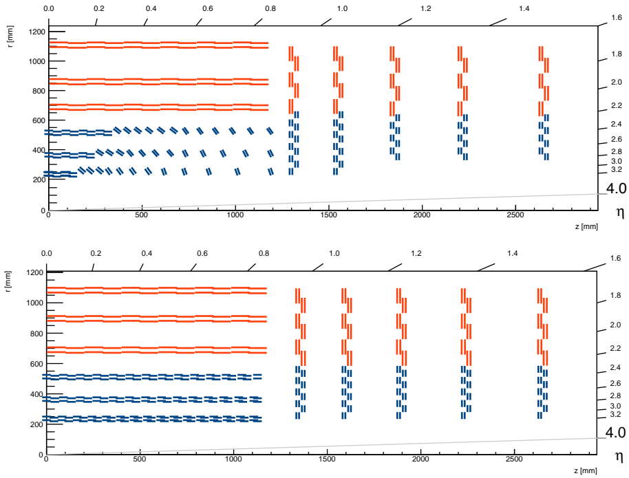
Figure 3. One quadrant of the upgraded Outer Tracker layout, showing the 2S (red) and PS (blue) module placement. The upper diagram shows the currently proposed layout, known as the tilted barrel geometry [5, 10]. The tilt of the modules in the three PS barrel layers improves overall performance and reduces construction costs. The lower diagram shows an older proposal for the layout, known as the flat barrel geometry [4], which was adopted for all the studies presented in this paper, except where stated otherwise.
