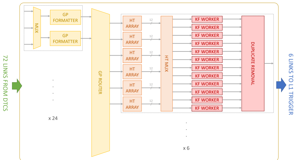
Figure 6. An overview of the TFP illustrating the main logic components and their interconnectivity, each described in detail in the text. Yellow components are part of the Geometrical Processor, orange components are part of the Hough Transform, red components are part of the Kalman Filter or Duplicate Removal. The TFP is capable of processing data from up to 72 input links (one per DTC). This allows for some margin in the exact number of DTCs, which is yet to be determined.
