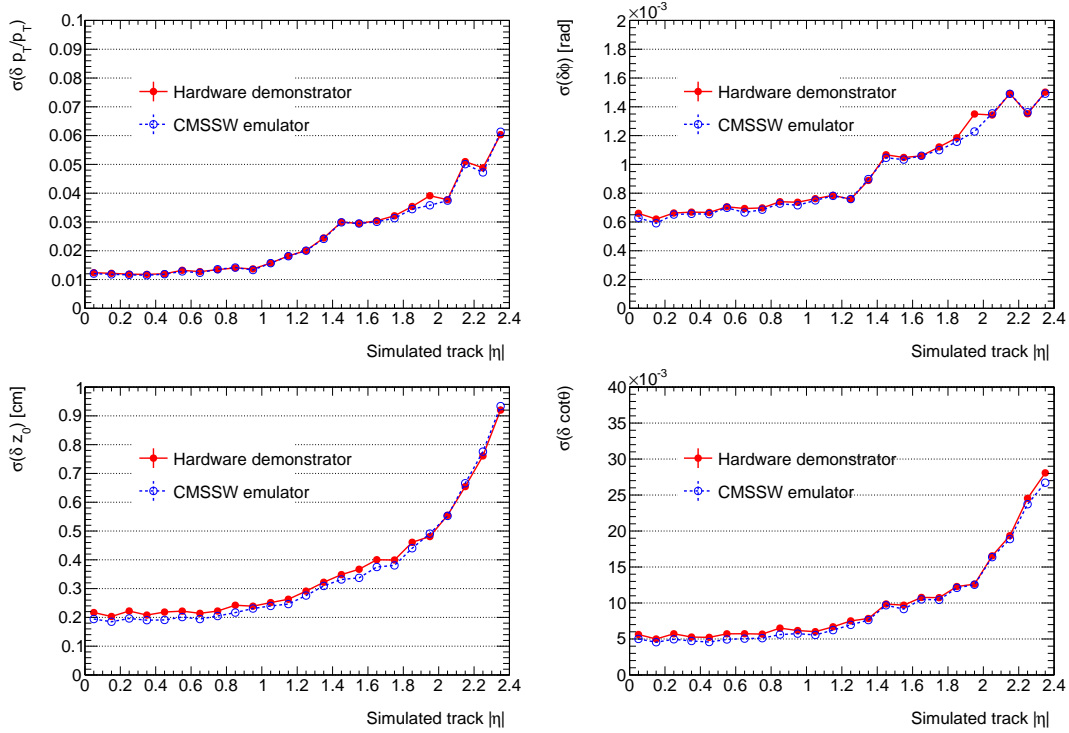
Figure 20. Relative p_T resolution, \phi resolution, z_0 resolution and \cot\theta resolution measured for tracks originating from the primary interaction in t\bar{t} events at PU of 200 as determined from both hardware and emulation.
