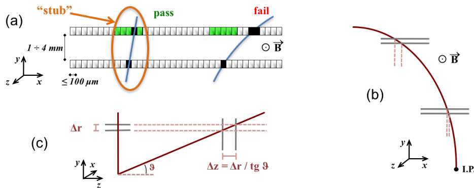
Figure 1. Cluster matching in p_T -modules to form stubs [5]. (a) Correlating pairs of closely-spaced clusters between two sensor layers, separated by a few mm, allows discrimination of transverse momentum. This is based on the bend of a particle’s trajectory in the CMS magnetic field and assumes that the particle originates at the beam line. (The beam-line is taken to be the line that passes through the centre of the luminous region and is parallel to the z -axis of the coordinate system, which in turn is parallel to both to the magnetic field and to the central axis of the CMS detector). Only stubs compatible with tracks with p_T > 2\text{--}3 GeV are transferred off-detector. (b) The separation between the two clusters increases with the module’s distance from the beam line, if the sensor spacing remains unchanged. (c) To achieve comparable discrimination in the endcap disks, which are orientated perpendicular to the beam-line, a larger sensor spacing is needed, because of projective effects.
