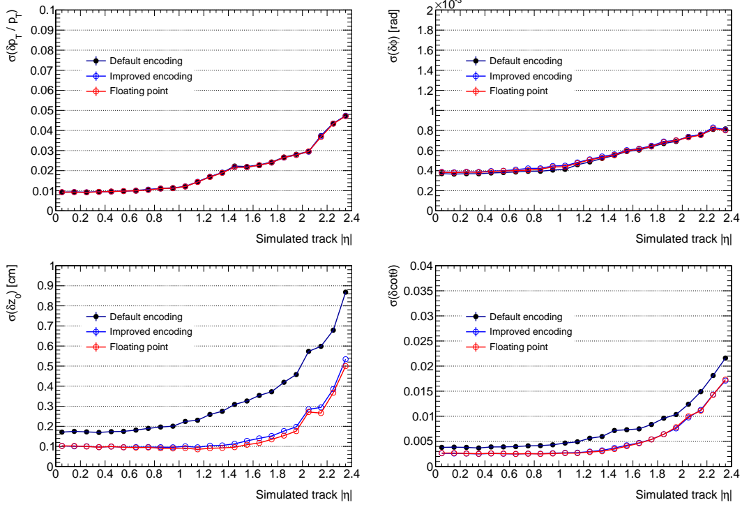
Figure 22. Relative p_T resolution, \phi resolution, z_0 resolution and \cot \theta resolution measured for single isolated muons with 5 < p_T^\mu < 15 GeV obtained from emulation, using different levels of precision in simulation: default encoding (10-bit r , 12-bit z , 15-bit \phi stub coordinates); improved encoding (12-bit r , 14-bit z , 15-bit \phi stub coordinates); and full floating-point simulation.
