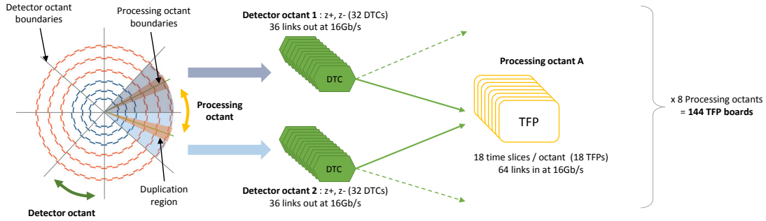
Figure 5. Baseline system architecture using DTCs in two neighbouring detector octants to time-multiplex and duplicate stub data across processing octant boundaries before transmission to the Track Finding Processors (TFPs). With 18 time nodes and eight processing octants, the full track finding system would be composed of 144 TFPs.
