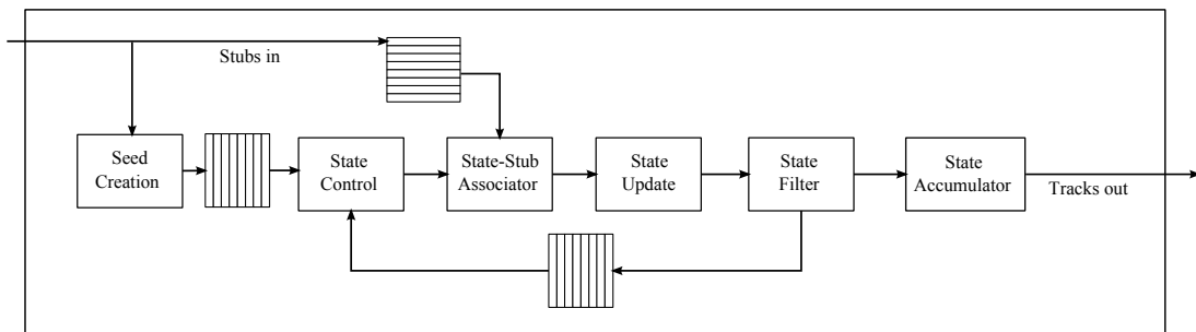
Figure 12. Connection of logical elements within a Kalman Filter worker.
