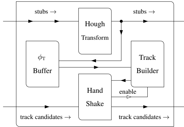
Figure 10. Firmware implementation of one Column, which corresponds to a single q/p_T column in the HT array. A number of Columns are daisy-chained together, starting and ending with the Book Keeper.
