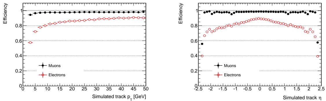
Figure 18. Track reconstruction efficiency, for electrons and muons from t\bar{t} events with 200 PU, as a function of p_T (left) and \eta (right). These results are obtained from emulation.
