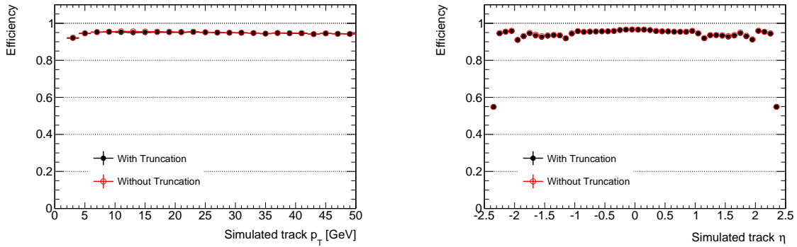
Figure 25. Track reconstruction efficiency for tracks originating from the primary interaction in t\bar{t} events with 200 PU, as a function of p_T (left) and \eta (right). These results are obtained from emulation both including and excluding truncation effects.
