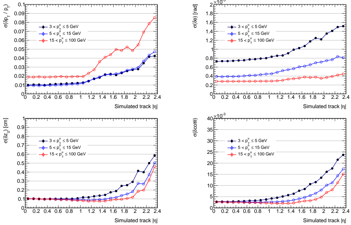
Figure 21. Relative p_T resolution, \phi resolution, z_0 resolution and \cot \theta resolution measured for single isolated muons with 3 < p_T^\mu < 5 GeV, 5 < p_T^\mu < 15 GeV, and 15 < p_T^\mu < 100 GeV. These results are obtained from emulation.
