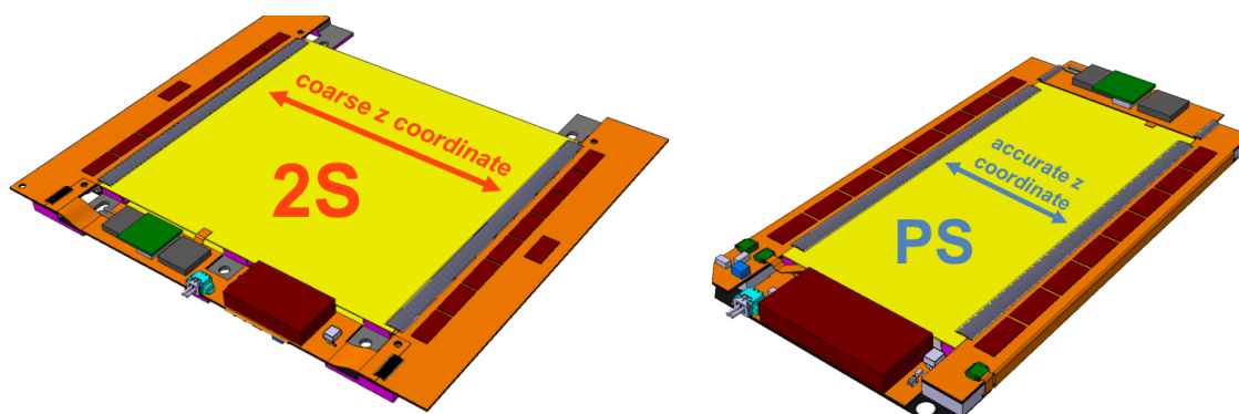
Figure 2. The 2S module (left) and PS module (right), described in the text [5]. Reproduced from [5]. CC BY 3.0.
