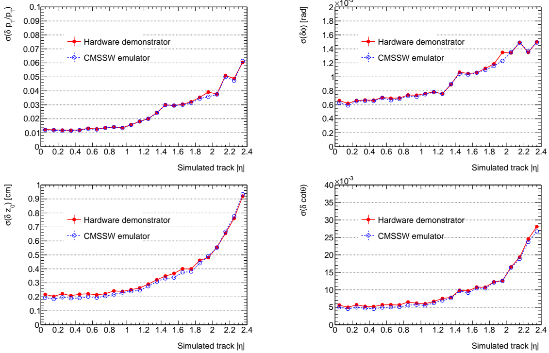
Figure 20. Relative p_T resolution, \phi resolution, z_0 resolution and \cot \theta resolution measured for tracks originating from the primary interaction in t\bar{t} events at PU of 200 as determined from both hardware and emulation.
