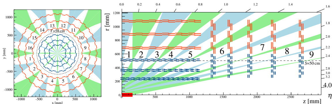
Figure 7. The segmentation of the tracker volume into \varphi sub-sectors (left) and \eta sub-sectors (right). The numbered areas in white represent the regions that are associated to only one sector, whereas the coloured areas (where there is no difference in meaning between green or blue) represent the overlap region between neighbouring sectors where stubs may need to be assigned to both sectors. The two cylinders mentioned in the text of radius T = 58 cm and S = 50 cm, are indicated by dashed lines in the left and right-hand figures, respectively.
