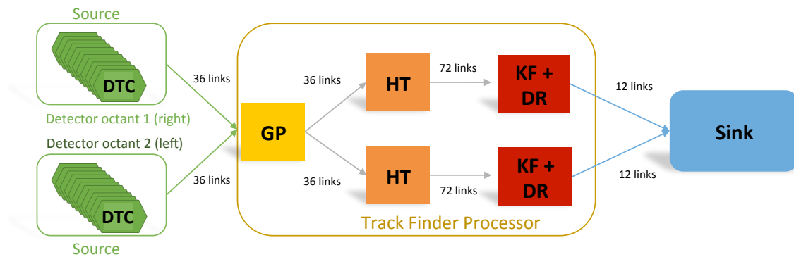
Figure 15. The demonstrator system consists of five layers of MP7s; source, Geometric Processor (GP), Hough Transform (HT), Kalman Filter + Duplicate Removal (KF+DR), and sink. A total of eight MP7-XE boards are used, each indicated by a separate coloured block in the diagram.
