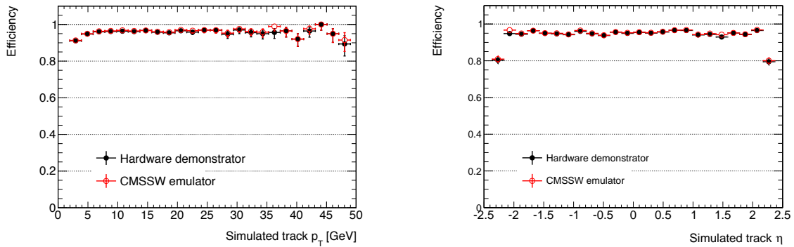
Figure 17. Track reconstruction efficiency, measured in both hardware and emulation, for tracks originating from the primary interaction in t\bar{t} events with 200 PU, as a function of p_T (left) and \eta (right).
