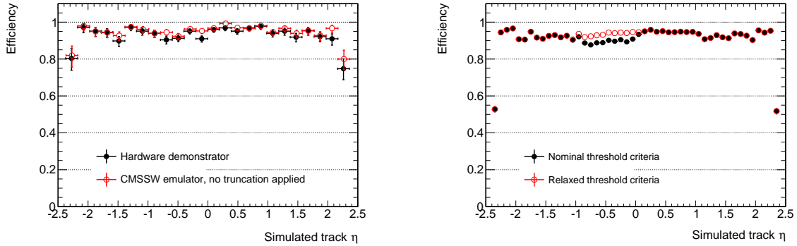
Figure 26. Left: track reconstruction efficiency as a function of \eta , measured in both hardware and emulation, when processing t\bar{t} events with 200 PU, where a global threshold criterion of four hit layers in the HT has been applied. To demonstrate the total efficiency loss due to truncation in hardware, the emulation result does not include truncation effects. Right: track reconstruction efficiency as a function of \eta , measured in emulation, when processing t\bar{t} events with 200 PU, where the tracker is affected by a failure of all modules in the region -1 < \eta < 0 and 0 < \varphi < \pi of barrel layer 4. Results are compared before (black dots) and after (red open circles) relaxing the threshold criterion on number of hit layers in the affected region, as described in the text.
