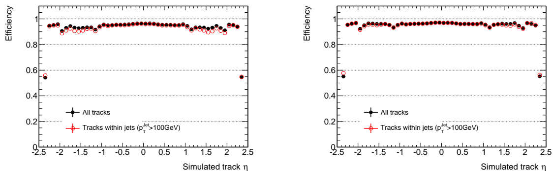
Figure 19. Track reconstruction efficiency as a function of \eta , for all tracks originating from the primary interaction (black dots), or for only the tracks contained within a primary jet that has a total transverse momentum exceeding 100 GeV (red open circles), for t\bar{t} events at 200 PU. Either no incorrect stubs are allowed on the track (left), or one incorrect stub is allowed on the track at most (right). These results are obtained from emulation.
