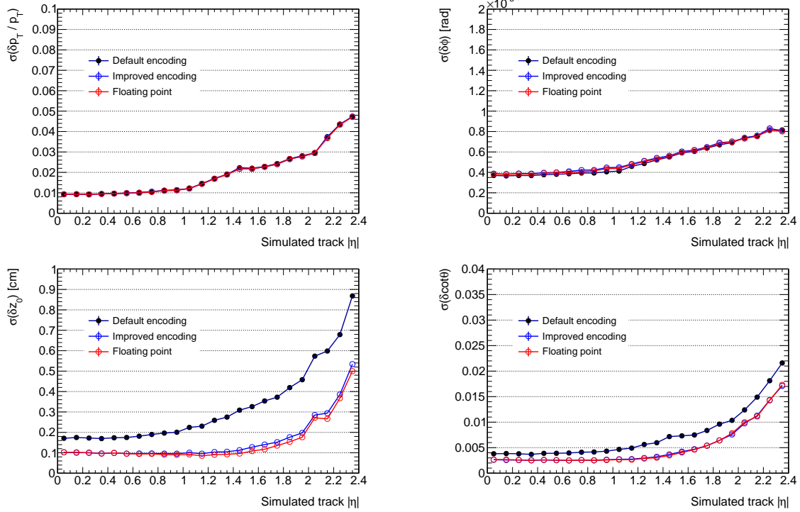
Figure 22. Relative p_T resolution, \phi resolution, z_0 resolution and \cot \theta resolution measured for single isolated muons with 5 < p_T^\mu < 15 GeV obtained from emulation, using different levels of precision in simulation: default encoding (10-bit r , 12-bit z , 15-bit \phi stub coordinates); improved encoding (12-bit r , 14-bit z , 15-bit \phi stub coordinates); and full floating-point simulation.
