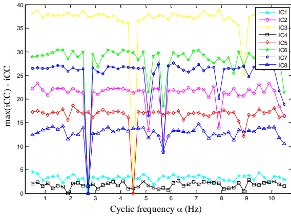
Fig. 4 (\max(iCC) - iCC) of independent components from JADE
