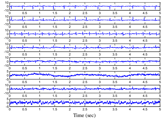
Fig. 6 Independent components extracted by FastICA from DaSy
