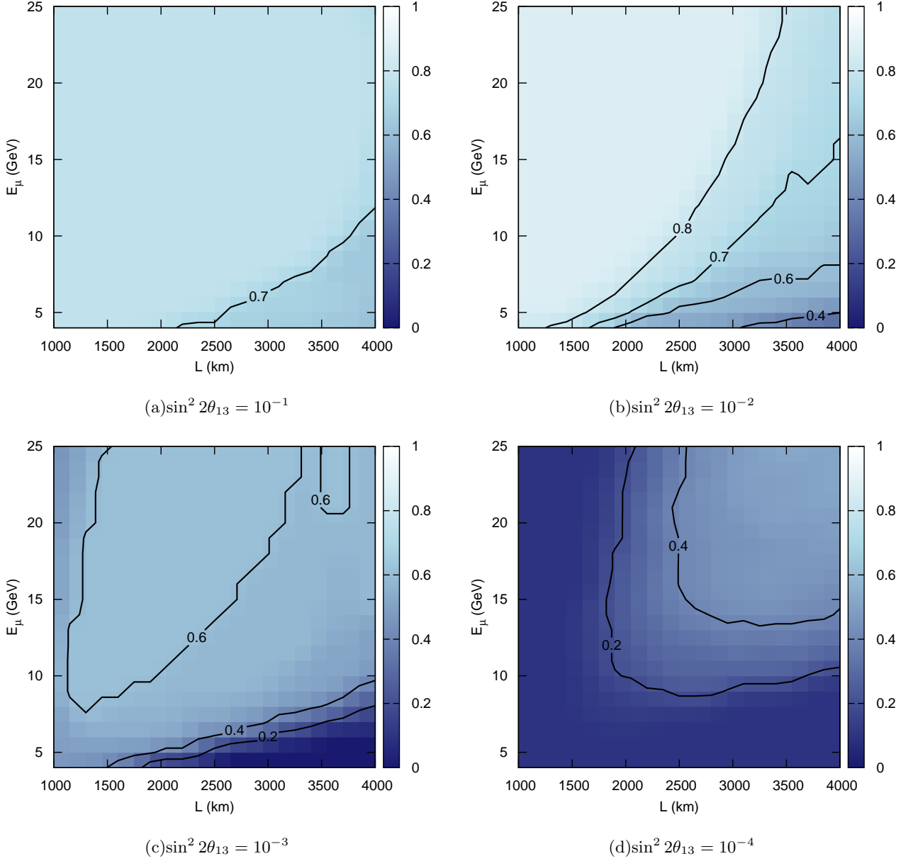
Figure 8. CP fraction as a function of baseline, L , and stored muon energy, E_\mu . Results are shown for a 20kTon TAsD using the default muon intensity of 5 \times 10^{21} \mu^+ and 5 \times 10^{21} \mu^- for four different values of \theta_{13} : (a) \sin^2 2\theta_{13} = 10^{-1} ; (b) \sin^2 2\theta_{13} = 10^{-2} ; (c) \sin^2 2\theta_{13} = 10^{-3} ; and (d) \sin^2 2\theta_{13} = 10^{-4} .
