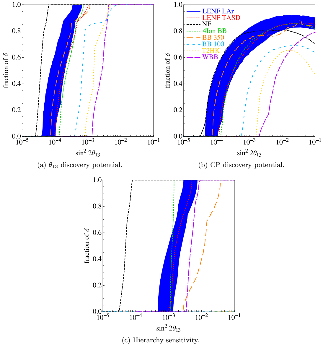
Figure 121. 3\sigma allowed contours for the LENF with 20 kton T ASD (red line) and 100 kton LAr detector (blue band), the HENF (black line), T2HK (yellow line), the wide-band beam (purple line) and three \beta -beams (green, orange, light blue lines) for a) \theta_{13} discovery potential, b) CP discovery potential and c) hierarchy sensitivity. From reference [116].
