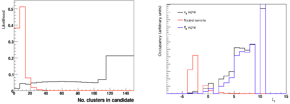
Figure 83. Number of clusters likelihood distribution function (left) and log-likelihood ratio (right) used to reject NC background. CC in black and NC in red.
