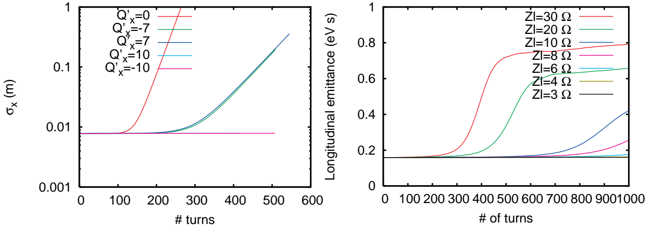
Figure 25. Horizontal beam size evolution, for various values of chromaticity, assuming a transverse impedance of 1 \text{ M}\Omega/\text{m} , Q_R=1 , f_R=1 \text{ GHz} (left). Longitudinal emittance evolution for different values of Z_{||}/n (right). The lines for 3 and 4 \Omega lie on top of each other in the figure.
