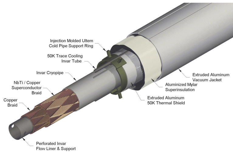
Figure 108. Schematic of superconducting transmission line showing construction details.
