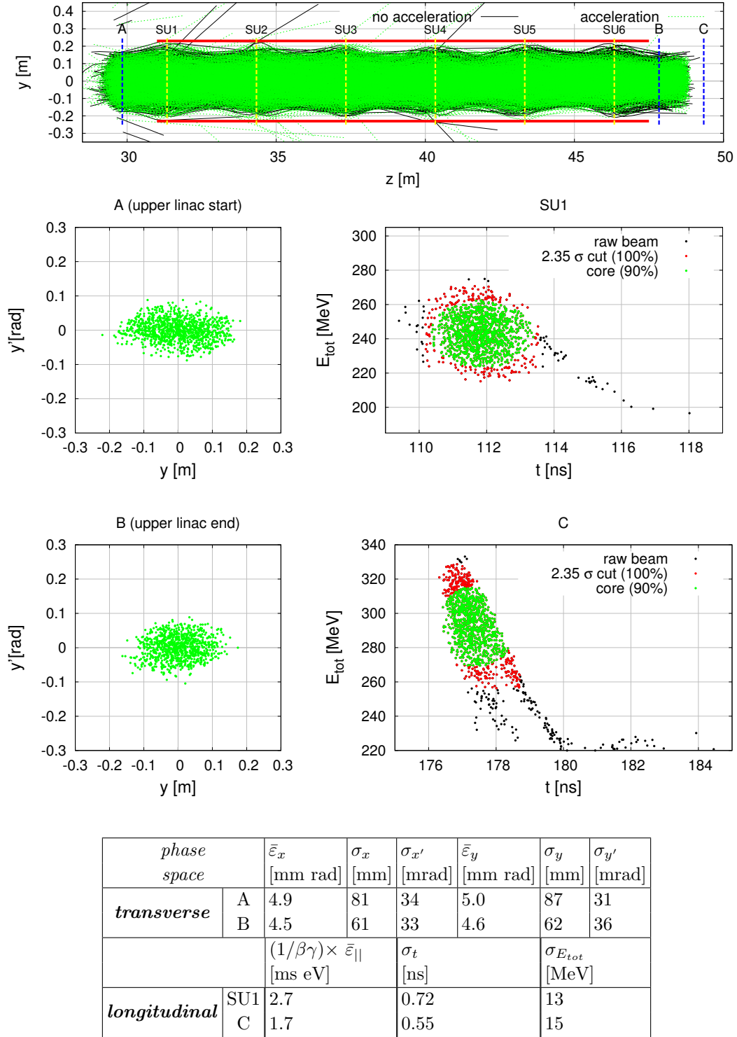
Figure 58. GPT particle trajectories through the upper linac (top), the y -phase space at its beginning/end (middle) and figures of the normalised emittances and standard deviations (bottom).
