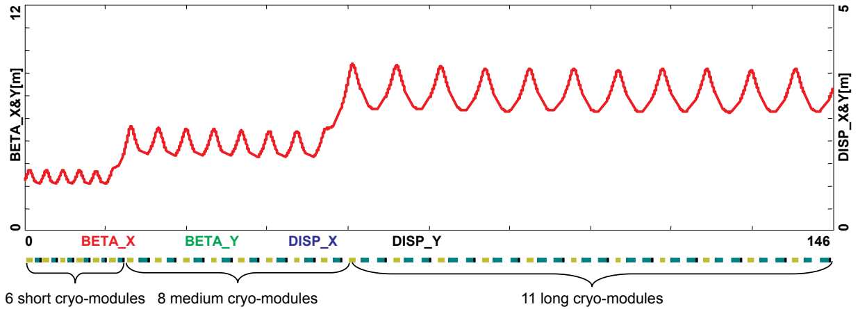
Figure 43. Transverse FOFO optics of the entire linac; the upper, middle and lower periodic sections uniformly matched at the junctions.
