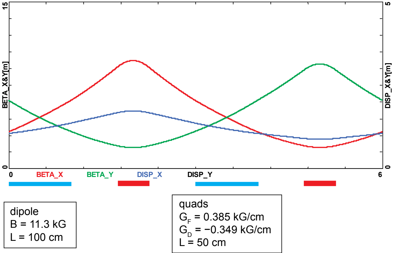
Figure 48. Periodic 90^\circ FODO 6 m inward-bending cell, including a pair of rectangular bends interleaved between quads. All elements are equally spaced.
