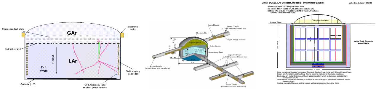
Figure 123. (left) GLACIER, (middle) JPARC-to-Okinoshima 100 kt concept and (right) 20 kt detector for DUSEL.
