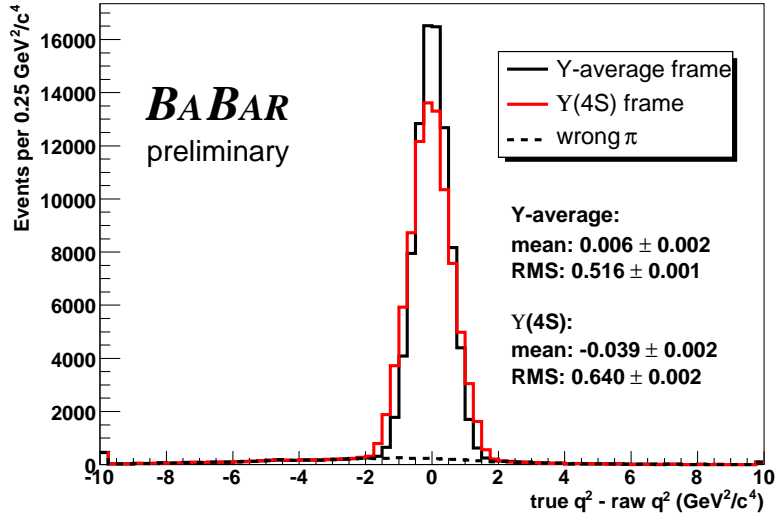
Figure 1: q^2 resolution of B^0 \rightarrow \pi^- \ell^+ \nu signal events obtained in the Y -average and Y(4S) frames after all analysis cuts and MC corrections. The very long tail arises when a track coming from the non-signal B is wrongly selected as the signal pion. The numbers of entries in the first and last bins correspond to the sum of all entries with \Delta q^2 < -9.75 \text{ GeV}^2/c^4 and \Delta q^2 > 9.75 \text{ GeV}^2/c^4 , respectively.
