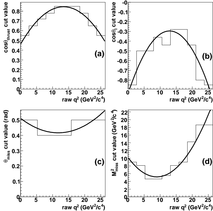
Figure 3: Cut functions used in the analysis, for the variables \cos\theta_{\text{thrust}} (a), \cos\theta_\ell (b), \theta_{\text{miss}} (c) and M_{\text{miss}}^2 (d). The solid curves show the cut values as a function of \tilde{q}^2 . The histograms show the statistically optimal cut values obtained in 10 \tilde{q}^2 bins based on the minimization of the quantity \sqrt{(S+B)}/S in the \Delta E - m_{\text{ES}} signal region, where S represents the simulated signal yield and B stands for the simulated background yield.
