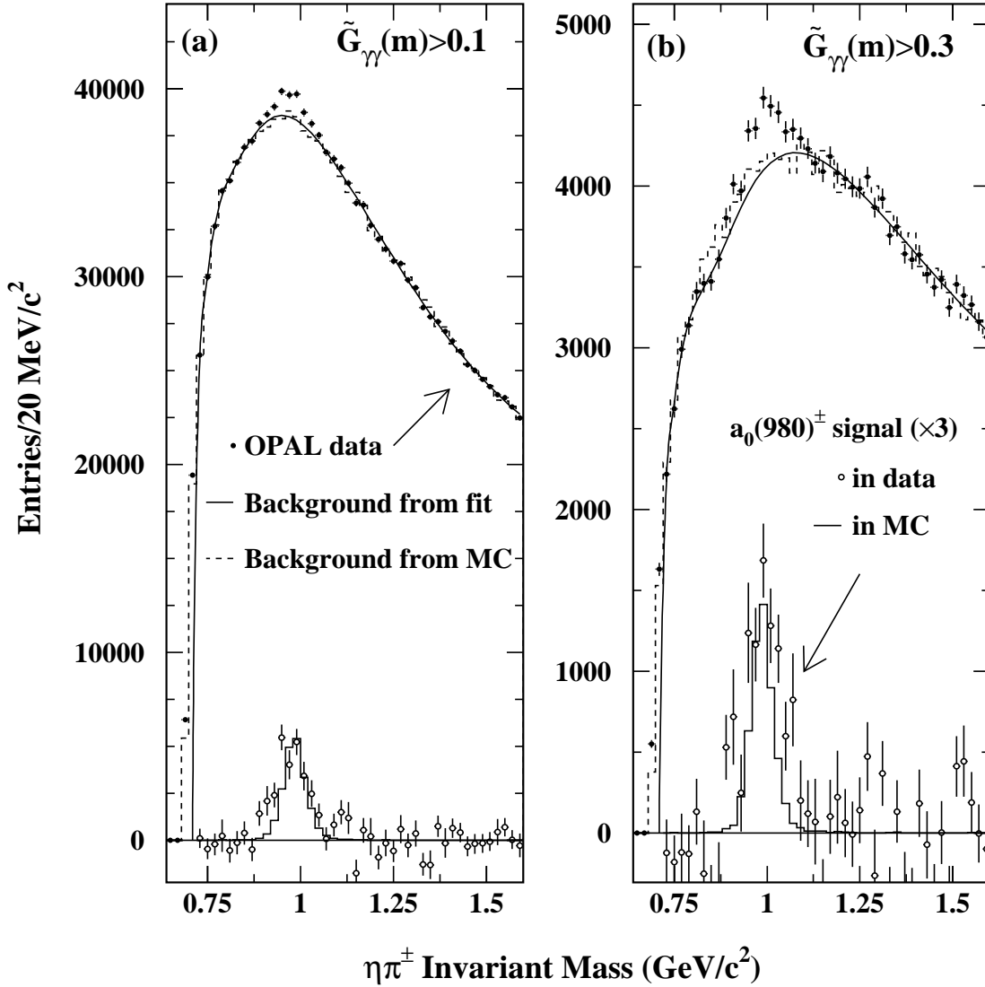
Figure 10: Fits to the invariant mass distribution of \eta\pi^{\pm} combinations for two different cuts on \tilde{G}_{\gamma\gamma}(m) . The points represent the OPAL data and the full curves the background obtained in the fit to the data. The dashed histograms correspond to the background evaluated using the Monte Carlo distributions. In the lower part of the figures, the signal obtained by subtracting the average of the two background from the data is shown as the open circles and is multiplied by a factor 3 for clarity. The full histogram is the Monte Carlo signal normalised to the same number of events.
