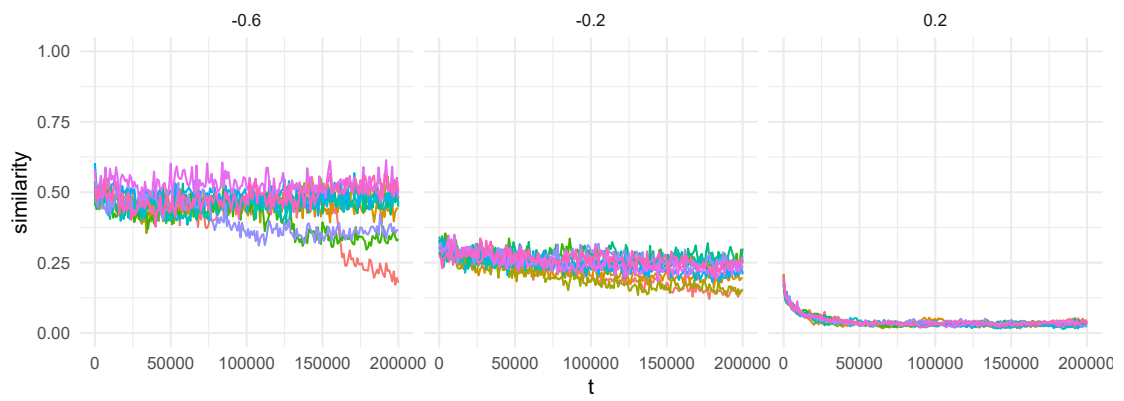
Figure 2: Average similarity over time, for ten simulation runs, between agents compared pairwise between two populations that were initially identical, for different average compatibilities in the trait pool.
