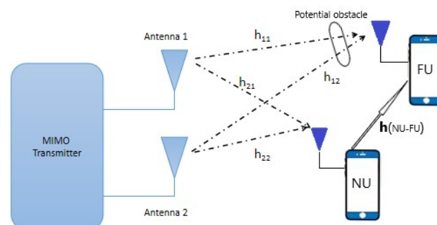
Figure 3. Cooperative SWIPT MIMO-NOMA in THz model.
