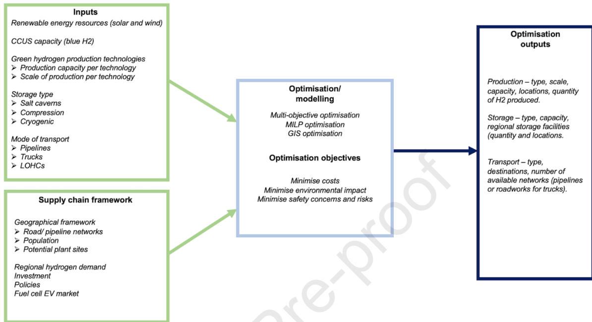
Figure 1: Optimising a hydrogen supply chain.
