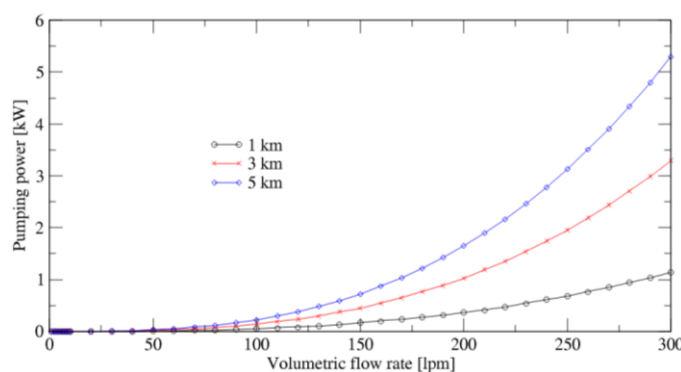
Fig. 3: Pumping power as a function of flow rate for various depths (VIT) and one year of operation.
