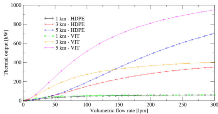
Fig. 2: Thermal output as a function of flow rate
