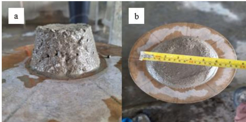
Figure 4. Flowability testing in progress.
