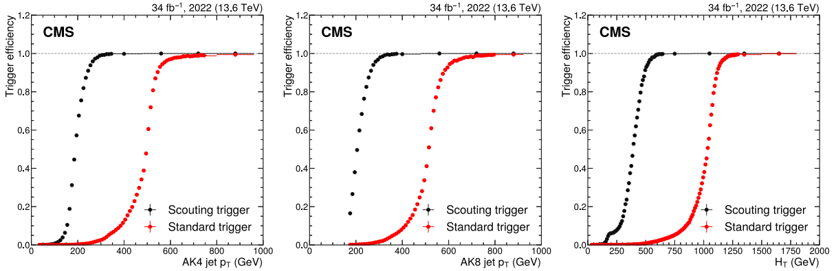
Fig. 26. Trigger efficiency as a function of AK4 jet p_T (left), AK8 jet p_T (center), and H_T (right). The efficiency is computed from collision data recorded in 2022 by the scouting (black points) and standard (red points) streams.
