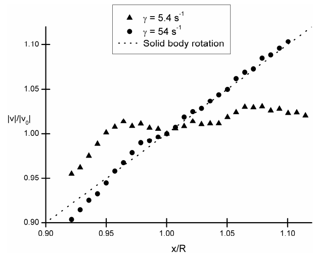
Fig. 6 Velocity magnitudes normalized by the velocity at centre of the viewing field for two different shear rates ( 5.4 and 54 \text{ s}^{-1} ) against normalised radius ( x/R ) at y=0 . Dotted line represents the expected velocity profile for solid body rotation.
