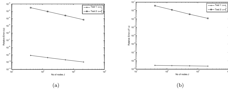
Figure 5. Relative error of the approximate solutions (a) and their gradients (b), on the circle vs. number of nodes J .
