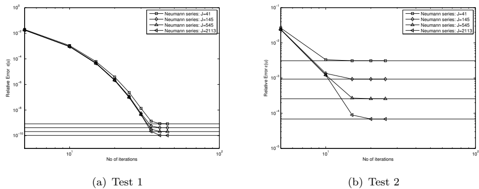
Figure 6. Relative error of the solutions on the circle domain vs. number of Neumann iterations, compared with the error of the LU decomposition solution (horizontal lines), for different number of mesh nodes J .
