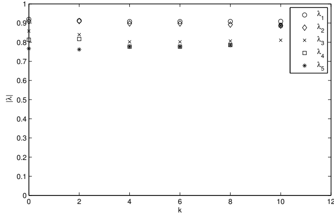
Figure 21. Moduli of the largest eigen-values of the matrix \hat{\mathbf{K}} for the parallelogram vs. k for a(x) = x^k_2 .
