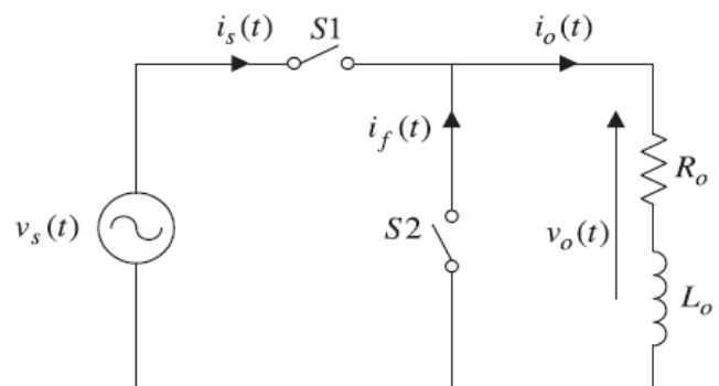
Fig. 01 - PWM AC/AC converter
