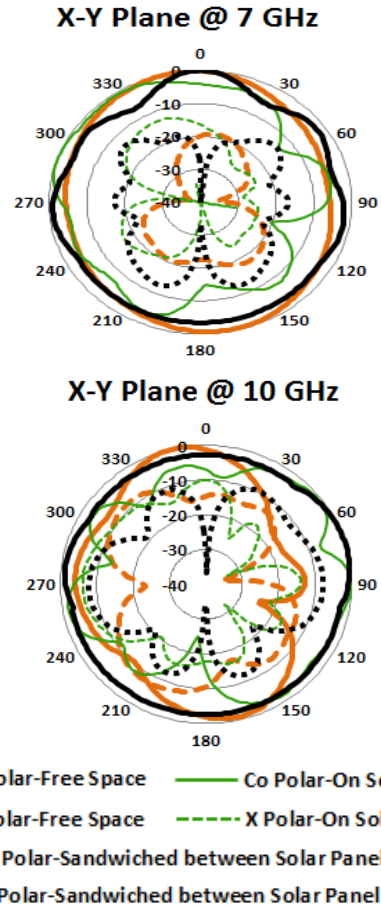
Fig. 10 Measured radiation patterns for CTSA in free space, on solar panel and sandwiched between a-Si solar panel and 2 mm glass at 3, 5, 7 and 10 GHz.
