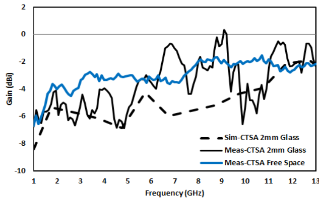
Fig. 15 Measured gain of CTSA on 2 mm glass substrate.
