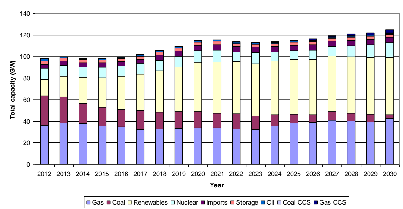
Figure 2. Total projected installed capacity by technology 2012-2030 [22].
