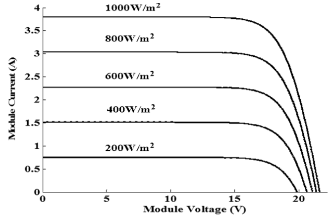
Fig. 3 I-V Characteristics with different irradiance values and a constant temperature ( 25^{\circ}\text{C} ).
