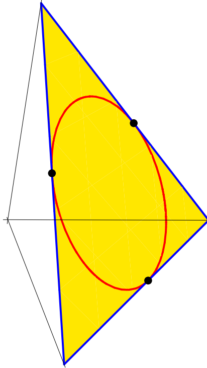
FIGURE 1. The image of the moment mapping \mu: \mathbb{CP}^2 \rightarrow \mathbb{R}^3 is a two-simplex \mathcal{T} that takes the form of a filled equilateral triangle. If \mathbf{z} = (z_1, z_2, z_3) is a unit vector in \mathbb{C}^3 , the point [\mathbf{z}] is mapped to (x_1, x_2, x_3) = (|z_1|^2, |z_2|^2, |z_3|^2) . The inscribed circle is the intersection of the plane x_1 + x_2 + x_3 = 1 containing the (coloured) image of \mu and the (invisible) sphere x_1^2 + x_2^2 + x_3^2 = \frac{1}{2} .
