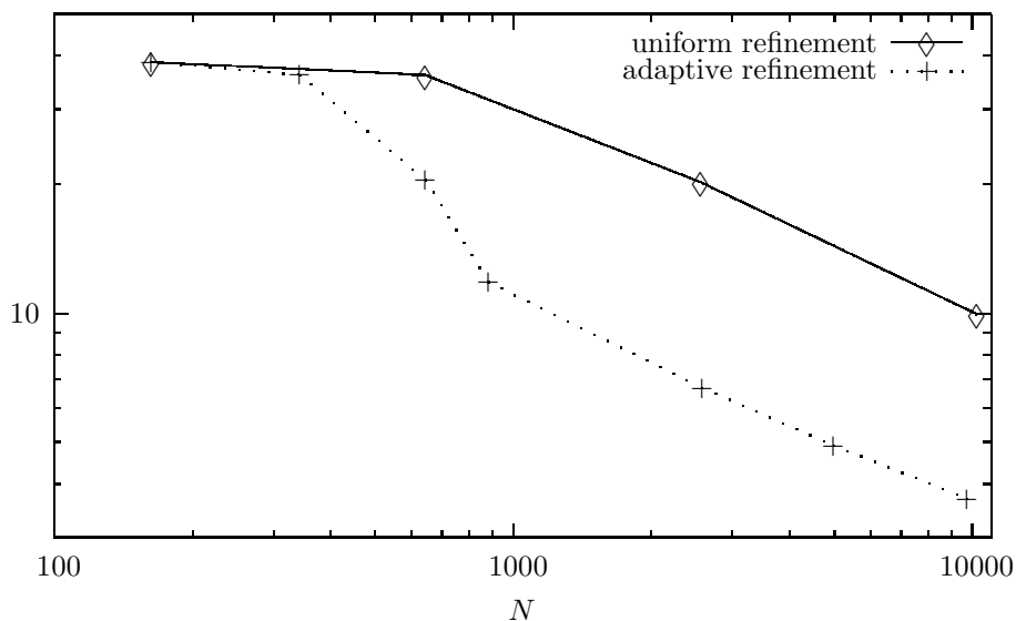
FIGURE 5.2. Total errors e(\boldsymbol{\sigma}, \mathbf{u}, \boldsymbol{\gamma}) vs. degrees of freedom N for the uniform and adaptive refinements (Ex. 4).
