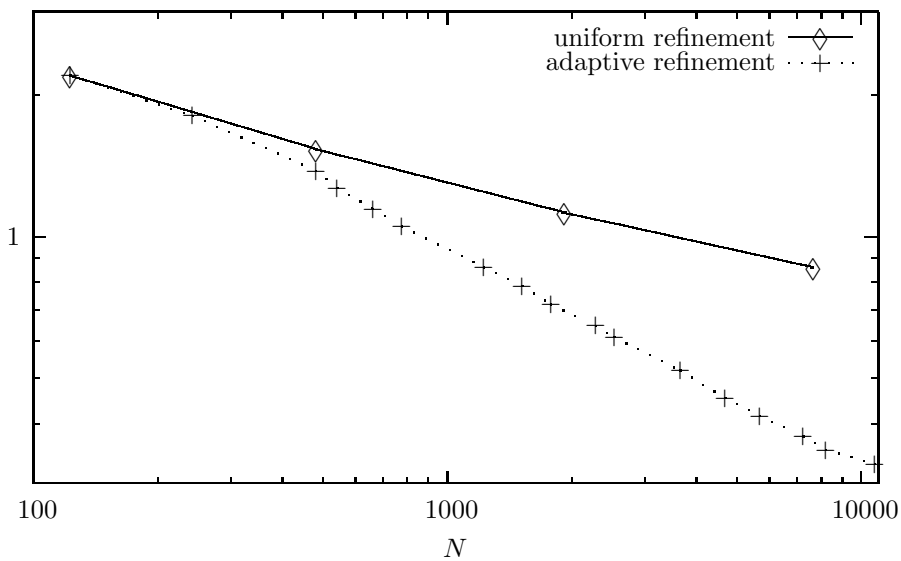
FIGURE 5.1. Total errors e(\boldsymbol{\sigma}, \mathbf{u}, \boldsymbol{\gamma}) vs. degrees of freedom N for the uniform and adaptive refinements (Ex. 3).
