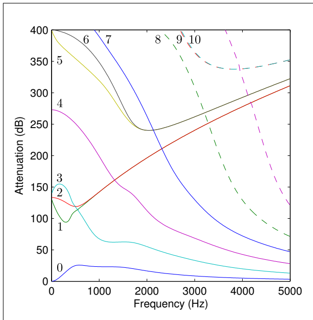
Figure 4. The least attenuated modes within the parallel baffle silencer.
