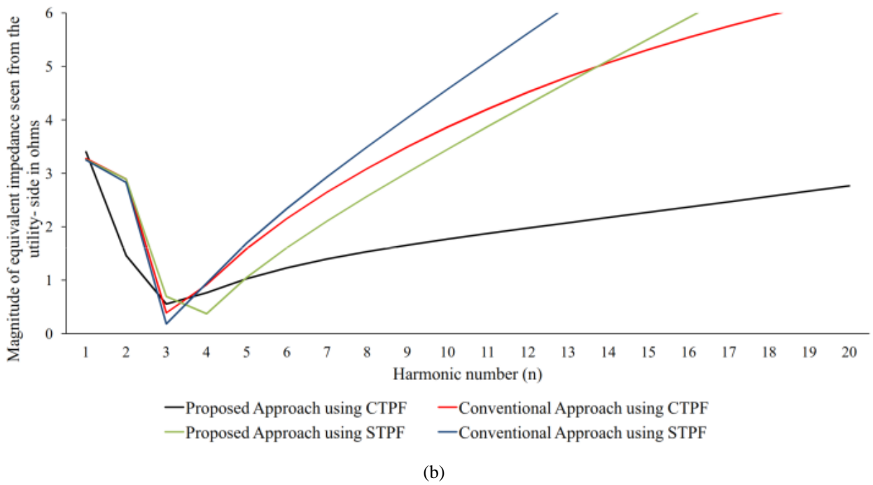
Fig. 5. The equivalent impedance seen from the utility- side versus harmonic number of both approaches using CTPF and STPF (a) Case 1 (b) Case 2
