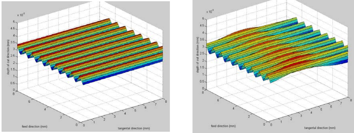
(a) Turning without taking account of non-linear factors (b) Turning with taking account of non-linear
