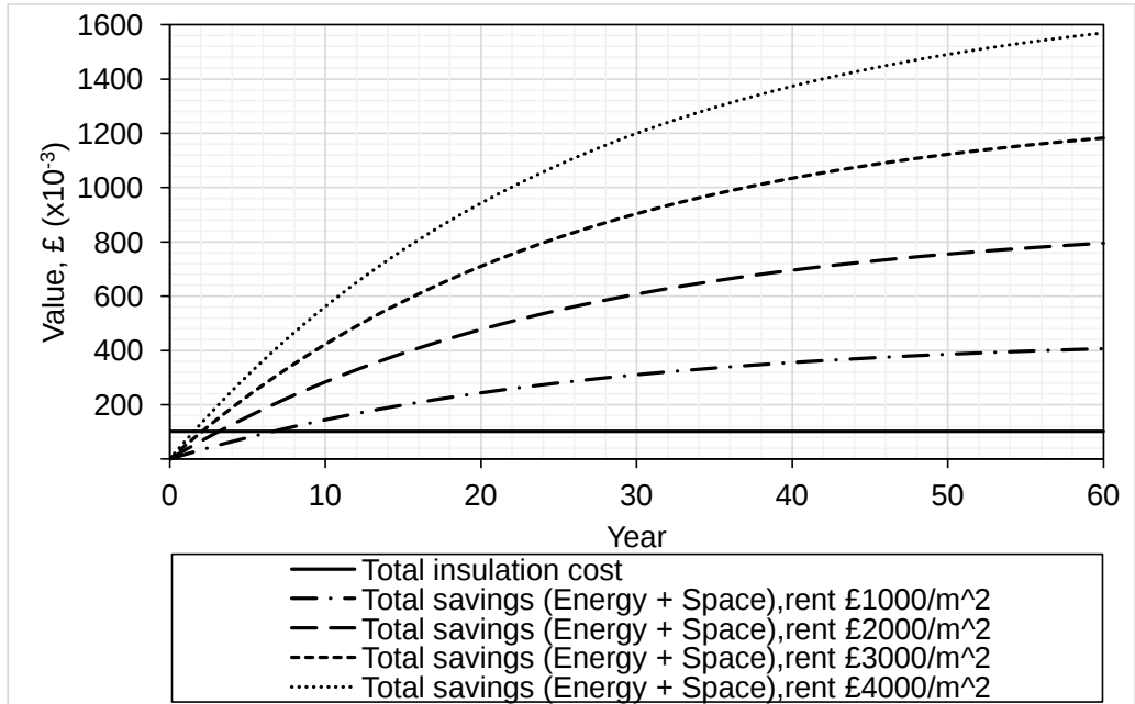
515 516 517 Figure 7. Cost and savings of applying GF VIP insulation in the retail unit building 518 studied 519
