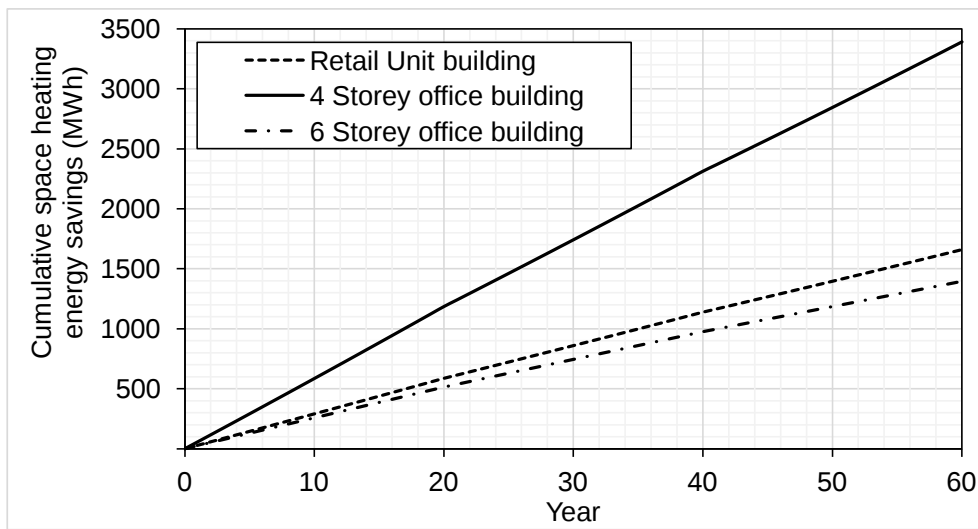
Figure 4. Cumulative space heating energy savings of the VIP insulated buildings studied
