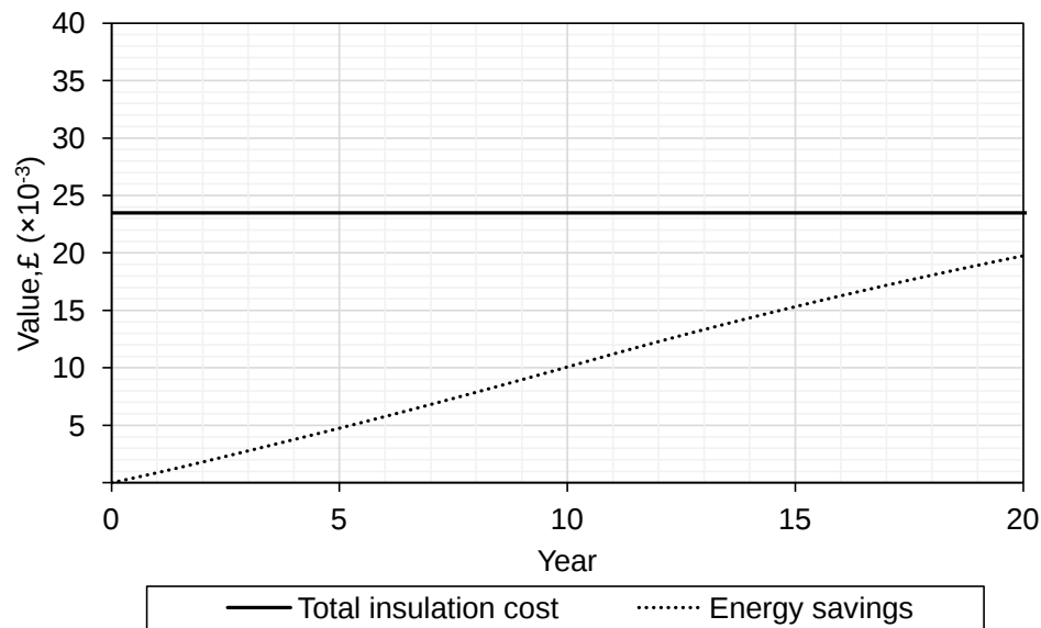
Figure 9. Cost and savings of applying EPS insulation in the 4 storey office building studied
