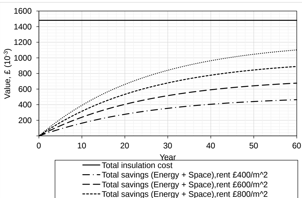
Figure 10. Cost and savings of applying CF-VIP insulation in the 4-storey office building studied
