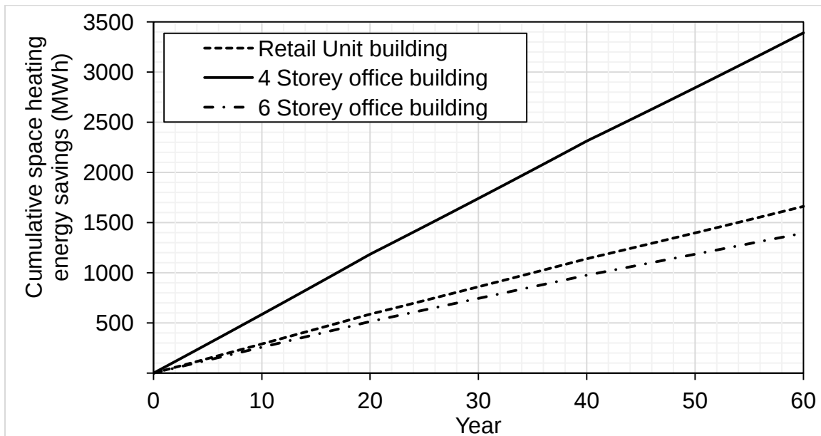
Figure 4. Cumulative space heating energy savings of the VIP insulated buildings studied
