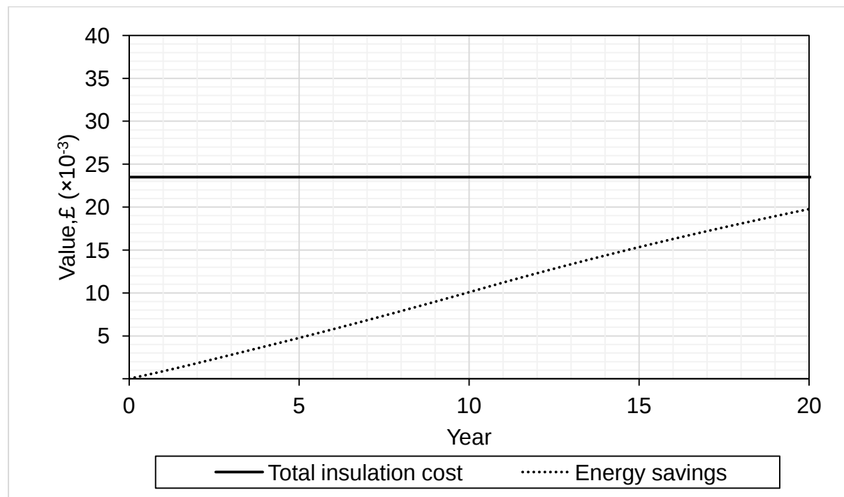
Figure 9. Cost and savings of applying EPS insulation in the 4 storey office building studied
