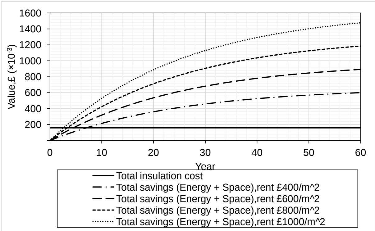
Figure 13. Cost and savings of applying GF VIP insulation in the 6 storey office building studied
