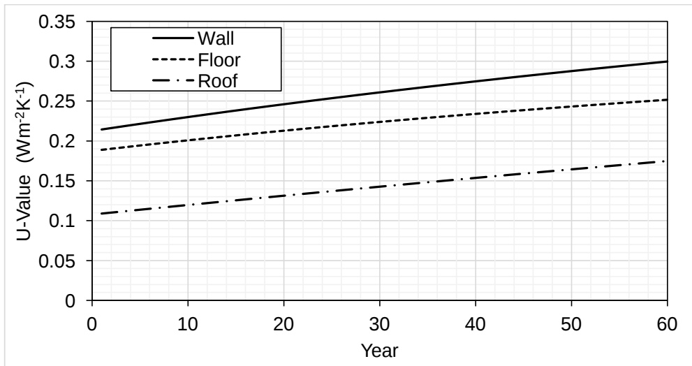
Figure 3. Time dependent U-values of VIP insulated wall, floor and roof of the two floor retail unit building studied
