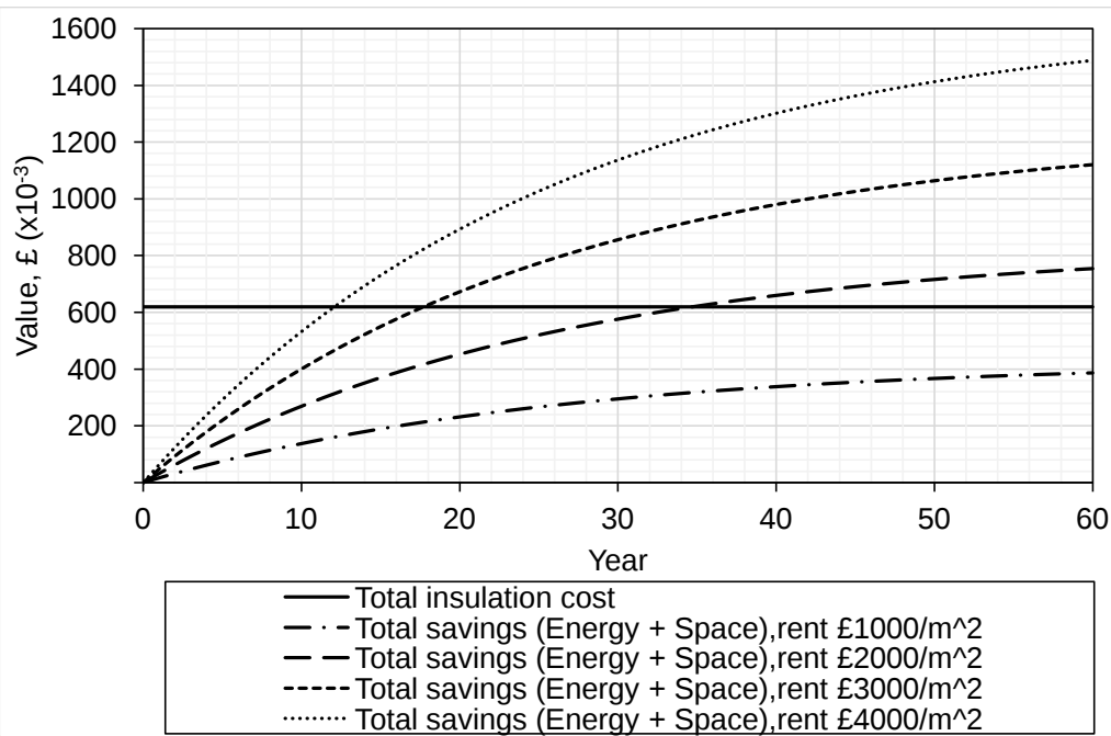
Figure 7. Cost and savings of applying GF VIP insulation in the retail unit building studied
