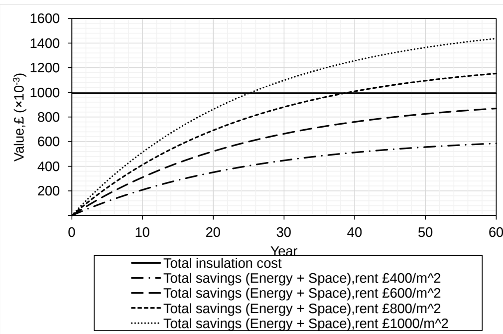
Figure 12. Cost and savings of applying EPS insulation in the 6 storey office building studied
