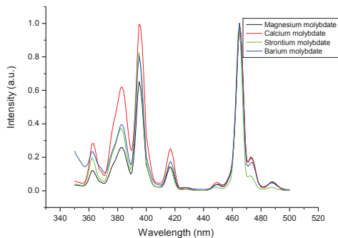
Fig. 3. Excitation spectra of the \text{Eu}^{3+} doped alkaline earth metal molybdates (350-500nm) normalised.
