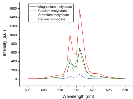
Fig. 5. Emission spectra of of the \text{Eu}^{3+} doped alkali earth metal molybdates excited at 465nm.
