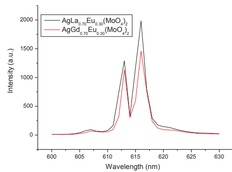
Fig. 7. Emission spectra of \text{AgLa}_{0.70}\text{Eu}_{0.30}(\text{MoO}_4)_2 and \text{AgGd}_{0.70}\text{Eu}_{0.30}(\text{MoO}_4)_2 , excited at 465 nm.
