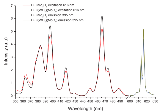
Fig. 8. Excitation and emission spectra of \text{LiEu}(\text{MoO}_4)_2 and \text{LiEu}(\text{MoO}_4)(\text{WO}_4) phosphors
