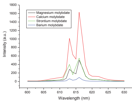
Fig. 4. Emission spectra of of the \text{Eu}^{3+} doped alkali earth metal molybdates excited at 395nm.
