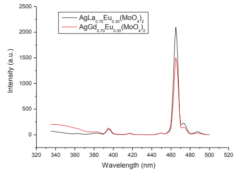
Fig. 6. Excitation spectra of \text{AgLa}_{0.70}\text{Eu}_{0.30}(\text{MoO}_4)_2 and \text{AgGd}_{0.70}\text{Eu}_{0.30}(\text{MoO}_4)_2 , monitored at 616 nm.
