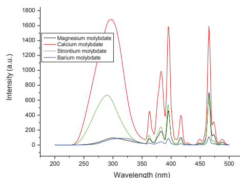
Fig. 1. Excitation spectra of the Eu 3+ doped alkaline earth metal molybdates
