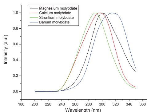
Fig. 2. Excitation spectra of the Eu 3+ doped alkaline earth metal molybdates (200-350nm) normalised.
