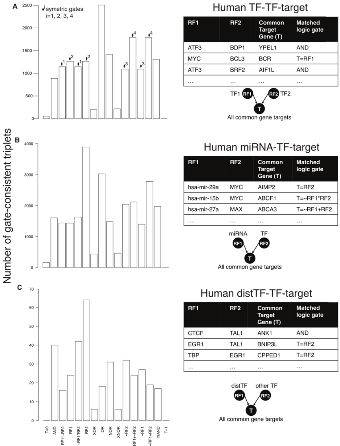
Fig 4. Distributions by logic gate of all gate-consistent human regulatory triplets in acute myeloid leukemia. A —TF-TF-target triplets. The symmetric gate pairs are marked using diamonds on top of bars with identical superscript numbers; B —miRNA-TF-target triplets; C —distTF-TF-triplets. The triplets from B and C have different distributions from A , including notably at symmetric gates because their RF1s are miRNA/distTF. Also, the “T = RF2” gate matches more triplets than any other gate in B and C .
