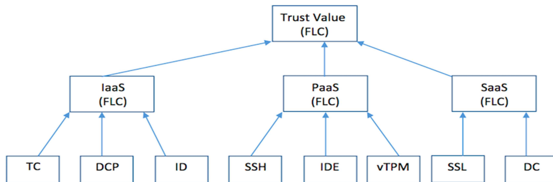
Fig. 1 MLSTM concept
