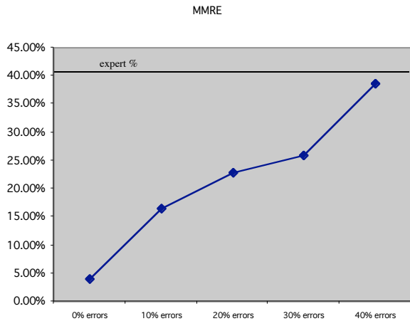
Figure 3: Prediction Accuracy Against Simulated Pairwise Comparison Error Rates
