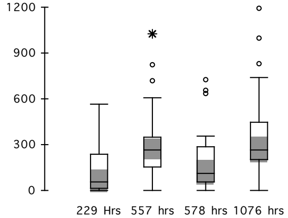
Figure 4a: Distribution of Prediction Errors using Different Reference Tasks (BT dataset)
