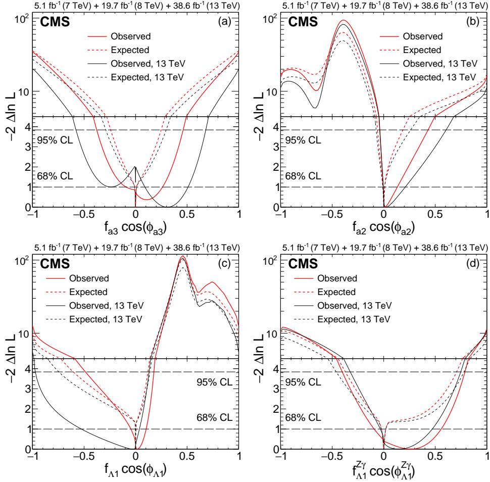
Figure 3: Observed (solid) and expected (dashed) likelihood scans of f_{a3} \cos(\phi_{a3}) (a), f_{a2} \cos(\phi_{a2}) (b), f_{\Lambda 1} \cos(\phi_{\Lambda 1}) (c), and f_{\Lambda 1}^{Z\gamma} \cos(\phi_{\Lambda 1}^{Z\gamma}) (d). Results of the Run 2 only and the combined Run 1 and Run 2 analyses are shown.
