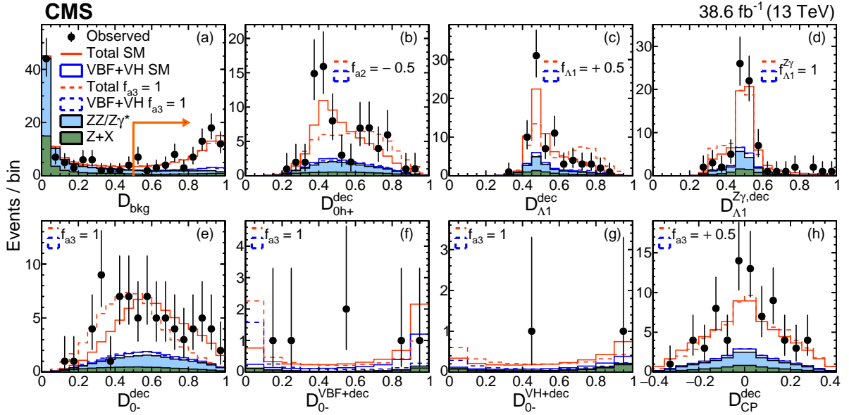
Figure 2: Distributions of \mathcal{D}_{\text{bkg}} (a) for all events in Run2; \mathcal{D}_{0h+} (b), \mathcal{D}_{\Lambda 1} (c), \mathcal{D}_{\Lambda 1}^{Z\gamma} (d), \mathcal{D}_{0-} (e), and \mathcal{D}_{CP} (h) for the untagged and 2015 events; \mathcal{D}_{0-} in the VBF-jet (f) and VH-jet (g) categories. The arrow in (a) indicates the requirement \mathcal{D}_{\text{bkg}} > 0.5 , used to suppress background on all other plots. Points with error bars show data and histograms show expectations for background and signal, as indicated in the legend in (a). The dashed lines show expectations for BSM hypotheses, as indicated in the individual legends.
