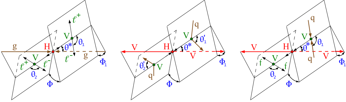
Figure 1: Illustration of H boson production and decay in three topologies: gluon fusion gg \rightarrow H \rightarrow VV \rightarrow 4\ell (left); vector boson fusion qq \rightarrow VV(qq) \rightarrow H(qq) \rightarrow VV(qq) (middle); and associated production qq \rightarrow V \rightarrow VH \rightarrow (ff)H \rightarrow (ff)VV (right). In the latter two cases, although the full H decay chain is not shown in the figure, the production and decay H \rightarrow VV may be followed by the same four-lepton decay shown in the first case. The five angles shown in blue and the invariant masses of the two vector bosons shown in green fully characterize either the production or the decay chain. The angles are defined in either the H or V boson rest frames [26, 33].
