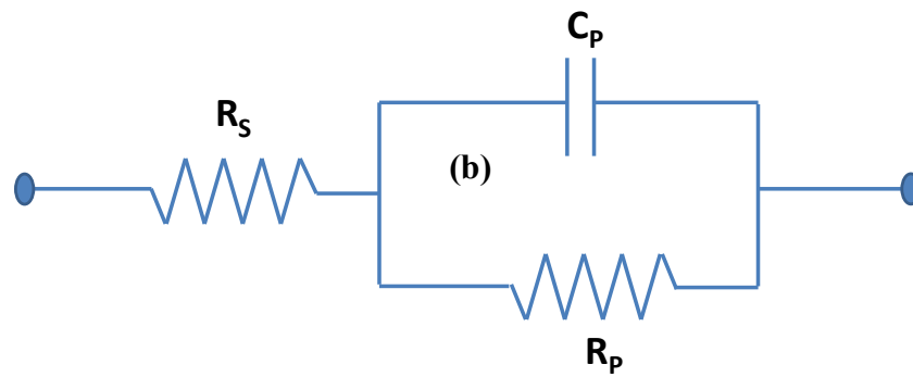
Figure 1. (a) Schematic FTO/TiO 2 / Perovskite/Pt structure for electrical measurement and (b) electrical equivalent circuit of the structure
