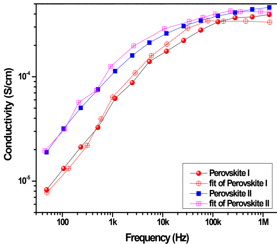
Figure 5. Conductivity vs frequency plots with fitted curve of Perovskite I and Perovskite II
