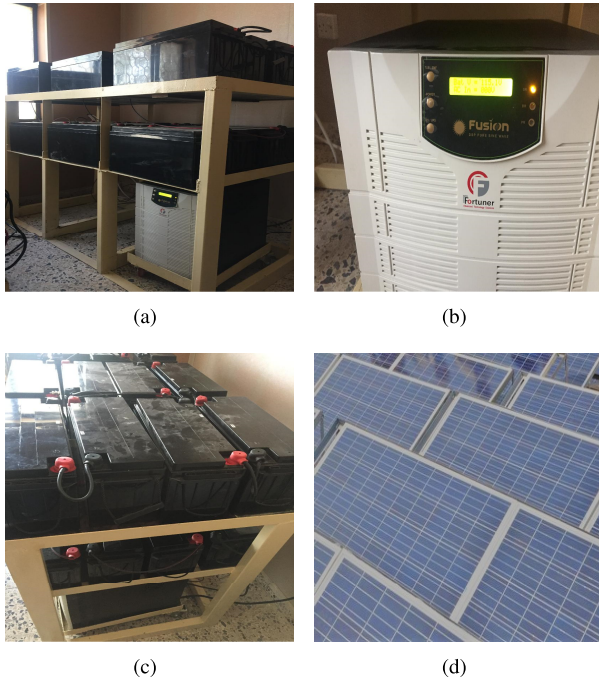
FIGURE 1. Solar system set up.
