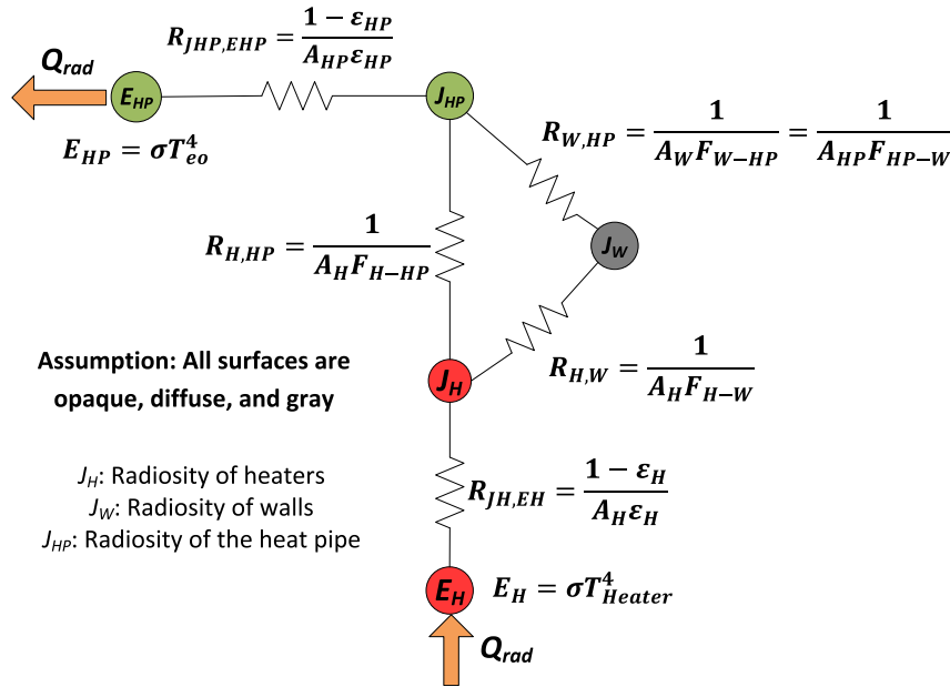
Fig. 15. Simplified thermal model of the radiation heat transfer in the kiln.
