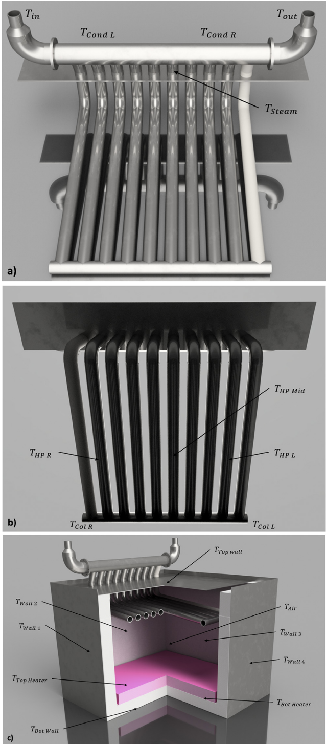
Fig. 11. Thermocouple locations.
