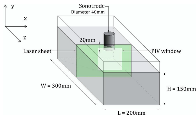
Fig. 1. Schematic of water tank for PIV measurements. The sonotrode is immersed 20 mm below the free surface of water at the axis of tank. Velocities are measured in a 2D 10 mm \times 10 mm window below the sonotrode.
