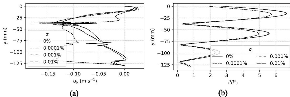
Fig. 10. (a) y -component of velocity and (b) acoustic pressure along the axis of the sonotrode from simulation corresponding to water with the transducer at 100% power as a function of bubble volume fraction averaged between 10 s and 20 s of simulation time. Positive velocities represent upflow.
