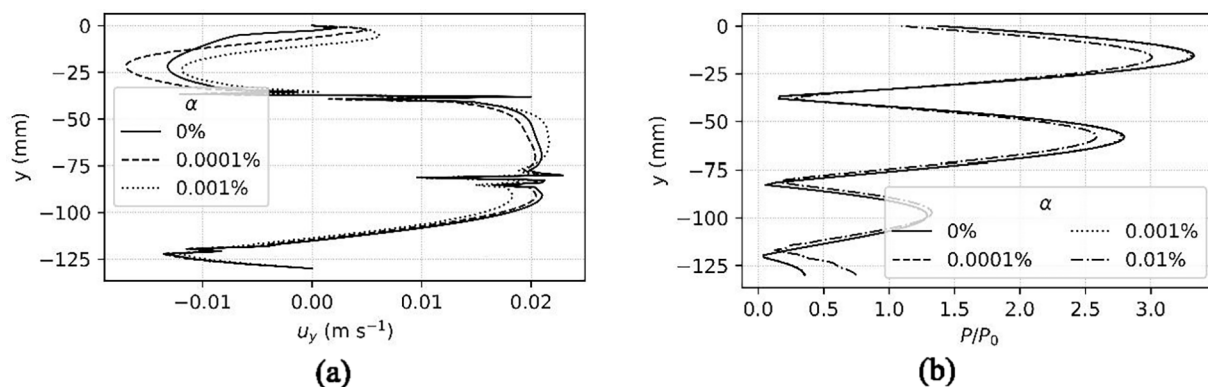
Fig. 6. (a) y -component of velocity and (b) acoustic pressure along the axis of the sonotrode from simulations corresponding to water with the transducer at 50% power as a function of bubble volume fraction averaged between 10 s and 20 s of simulation time. Positive velocities represent upflow. Note that the peaks in the predicted y components of velocity correspond to corresponding regions of high acoustic pressure gradients: these peaks are predicted because the driving force f from Eq. (14) is computed from acoustic pressure gradients.
