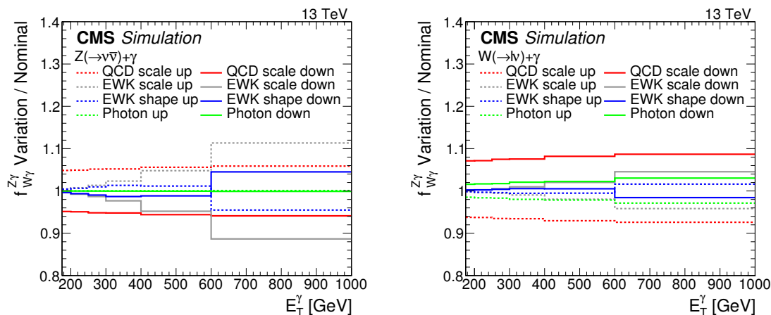
Figure 13. Systematic uncertainty in the transfer factors for Z(\rightarrow\nu\bar{\nu})+\gamma (left) and W(\rightarrow\ell\nu)+\gamma (right). The last bin includes all events with E_T^\gamma > 1000 GeV.
