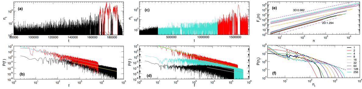
Figure 3. Signal selection according to the avalanche sizes for L = 256 , l = 32 (a,b), and according to three hysteresis-loop segments for l = L = 512 (c,d). The lower panel in each case shows the corresponding power spectrum of the selected signals against frequency f with the slopes \phi = 1.84 \pm 0.02 and 1.67 \pm 0.02 , panel (b), and \phi = 1.835 \pm 0.014 , 1.673 \pm 0.008 , and 1.208 \pm 0.009 , panel (d). Second-order fluctuation function F_2(n) vs segment length n for L = 512 and varied thickness l = 512 top line to l = 1 bottom line (e); the two dashed lines have the slopes equal to the Hurst exponent H(2) in 2D and 3D case. Distributions of the height n_t of the BHN signal for L = 256 and varied thickness l indicated in the legend, and a tangent—dashed line, (f).
