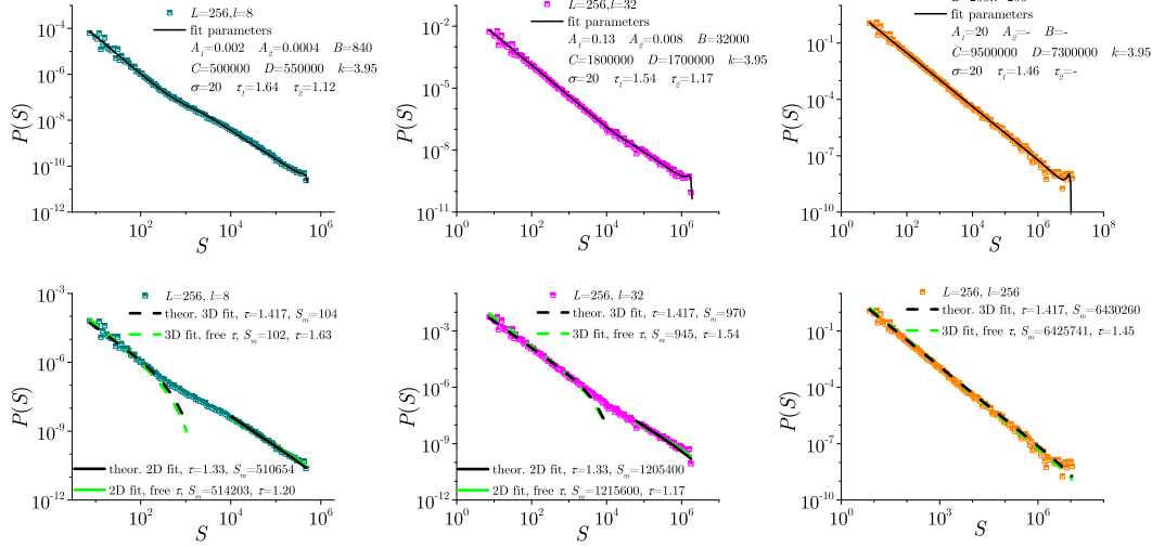
Figure 5. In the central part of the hysteresis loop, the distribution of avalanche size P(S) for different thickness l = 8, 32 , and 256 is fitted using the expression (4), top row, and the theoretical expression predicted for interface dynamics 48–50 , where 2D and 3D parts of the distribution are fitted separately, bottom row.
