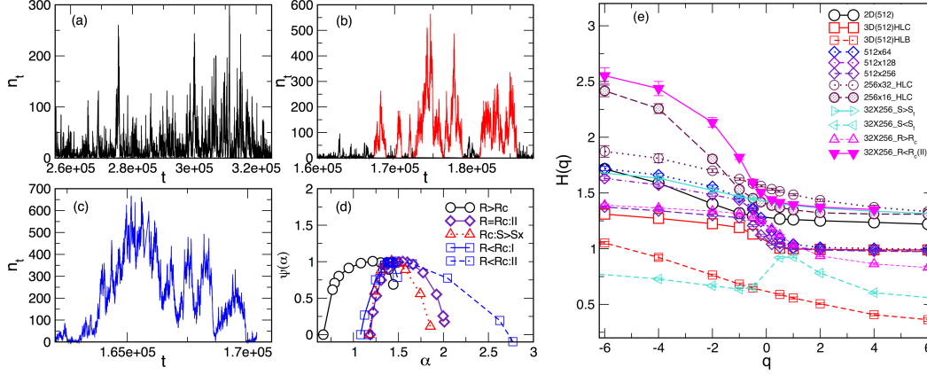
Figure 9. (a-c) Noise signal in the central part of HL for R > R_c , R = R_c , and R < R_c at the transitional sample thickness l_r = 32 for L = 256 and the corresponding effective critical disorder, for simplicity denoted by R_c . (d) The singularity spectra corresponding to these signals and indicated interval range, together with the spectrum referring to large avalanches selection, S > S_x . (e) Generalised Hurst exponents H(q) against q for all signals studied in Figs. 6, 7, and 8.
