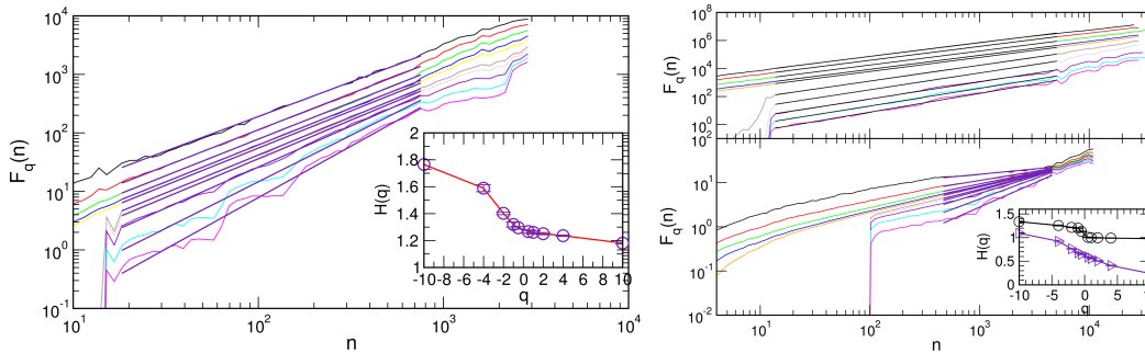
Figure 6. Fluctuation function F_q(n) for different values of q \in [-10, 10] for the whole signal for the 2D sample of size L = 512 (left panel), and 3D sample in the HLC (right, upper panel) and the initial segment of the loop (right, lower panel). Insets: corresponding generalised Hurst exponents H(q) against the amplification parameter q , see text.
