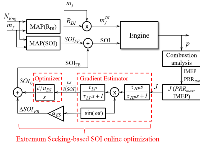
Fig. 13 Proposed control structure for DI fraction and SOI timing.
