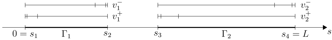
Figure 3: Illustration of the overlapping geometrically graded meshes used to approximate the amplitudes v_j^\pm in (34), in the case where \Gamma comprises two components, \Gamma_1 and \Gamma_2 .
