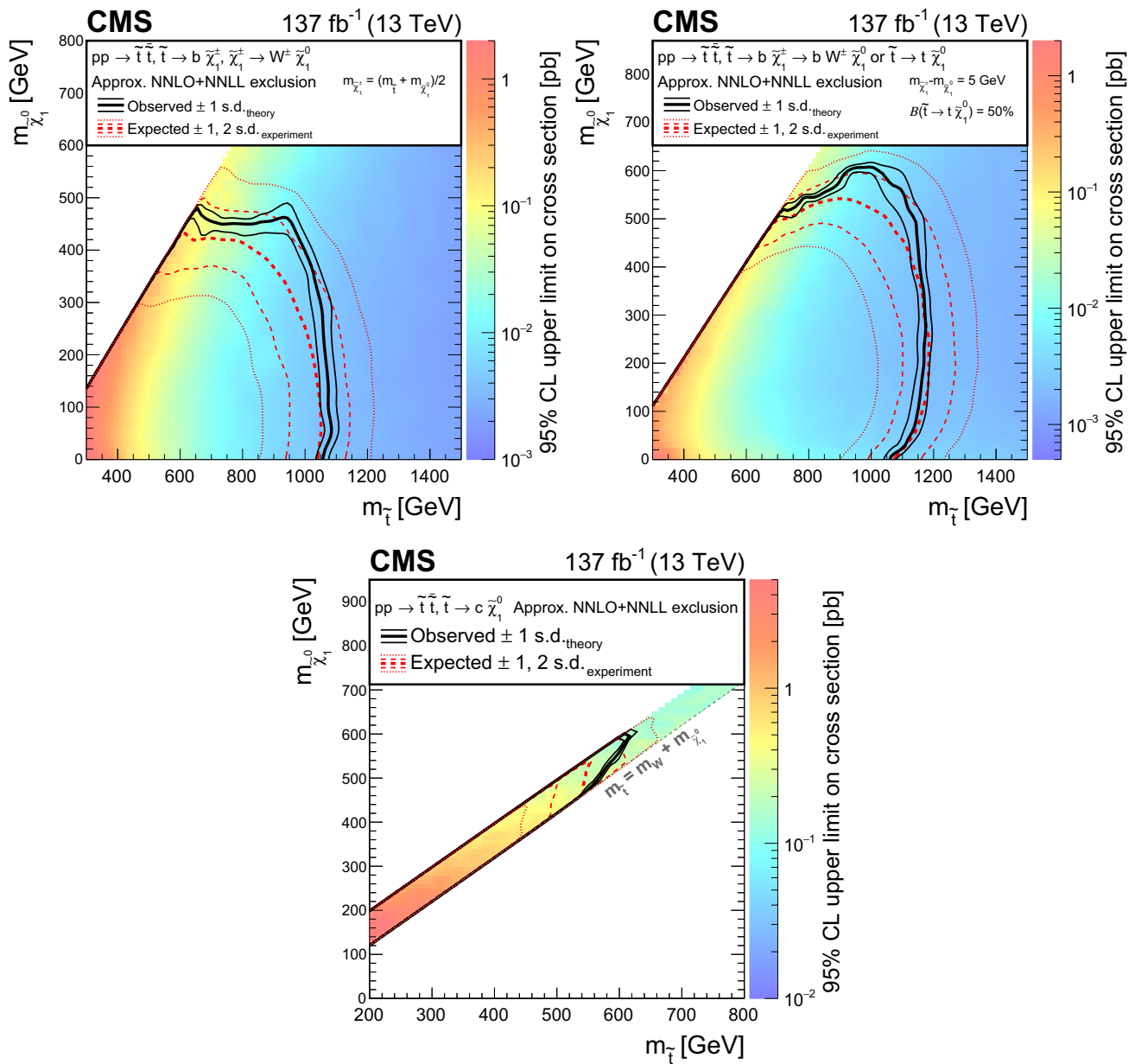
Fig. 14 Exclusion limit at 95% CL for top squark pair production for different decay modes of the top squark. (Upper left) For the scenario where pp \rightarrow \bar{t}t \rightarrow b\bar{b}\bar{\chi}_1^+\chi_1^+ , \bar{\chi}_1^{\pm} \rightarrow W^{\pm}\bar{\chi}_1^0 , the mass of the chargino is chosen to be half way in between the masses of the top squark and the neutralino. (Upper right) A mixed-decay scenario, pp \rightarrow \bar{t}t with equal branching fractions for the top squark decays \bar{t} \rightarrow t\bar{\chi}_1^0 and \bar{t} \rightarrow b\bar{\chi}_1^+ , \bar{\chi}_1^+ \rightarrow W^{*+}\bar{\chi}_1^0 , is also considered, with the chargino mass chosen such that \Delta m(\bar{\chi}_1^{\pm}, \bar{\chi}_1^0) = 5 GeV. (Lower) Finally, we also consider a compressed spectrum scenario where pp \rightarrow \bar{t}t \rightarrow c\bar{c}\bar{\chi}_1^0\bar{\chi}_1^0 . In this scenario,
