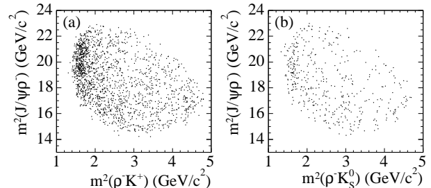
FIG. 2: The m^2(J/\psi\rho^-) versus the m^2(\rho^-K^+) distributions (a) for B^0 \rightarrow J/\psi\pi^-\pi^0K^+ and the m^2(J/\psi\rho^-) versus the m^2(\rho^-K_S^0) distributions (b) for B^- \rightarrow J/\psi\pi^-\pi^0K_S^0 . A B \rightarrow J/\psi K_1 signal can be seen, however there is no indication for an enhancement in the J/\psi\rho^- mass spectrum.
