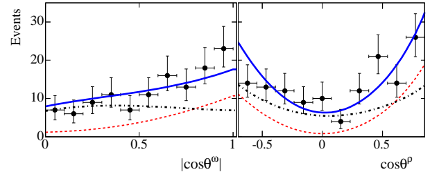
FIG. 2: Projections of helicity-angle cosines, of events passing a signal likelihood threshold for \omega (left) and \rho^+ (right) from the fit for B^+ \rightarrow \omega\rho^+ decay. The solid curve is the fit function, the dashed curve is the signal contribution, and the dot-dashed curve is the background contribution.
