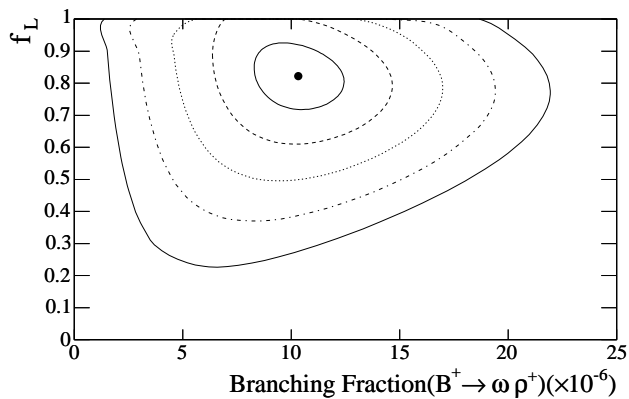
FIG. 3: Distribution of -2\ln\mathcal{L}(f_L, \mathcal{B}) for B^+ \rightarrow \omega\rho^+ decay. The solid dot gives the central value; curves give the contours in 1-sigma steps ( \Delta\sqrt{-2\ln\mathcal{L}(f_L, \mathcal{B})} = 1 ).
