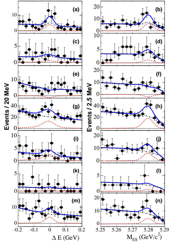
FIG. 1: Projections of \Delta E (left) and m_{ES} (right) of events passing a signal likelihood threshold for B^0 \rightarrow \omega K^{*0} , (a,b), B^+ \rightarrow \omega K^{*+} , (c,d), B^0 \rightarrow \omega\rho^0 , (e,f), B^+ \rightarrow \omega\rho^+ , (g,h), B^0 \rightarrow \omega\omega , (i,j), B^0 \rightarrow \omega\phi , (k,l) and B^0 \rightarrow \omega f_0 , (m,n). The solid curve is the fit function, the dashed curve is the signal contribution, and the dot-dashed curve is the background contribution.
