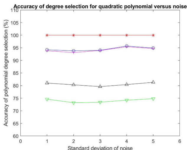
FIGURE 3. The accuracy (%) of degree selection using AIC (green lower triangles), AICc (black upper triangles), GIC (magenta + signs), BIC (blue circles), and PTS1 (red stars) versus noise standard deviations for a quadratic polynomial.
