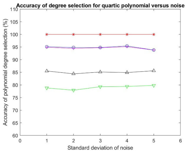
FIGURE 7. The accuracy (%) of degree selection using AIC (green lower triangles), AICc (black upper triangles), GIC (magenta + signs), BIC (blue circles), and PTS1 (red stars) versus noise standard deviations for a quartic polynomial.
