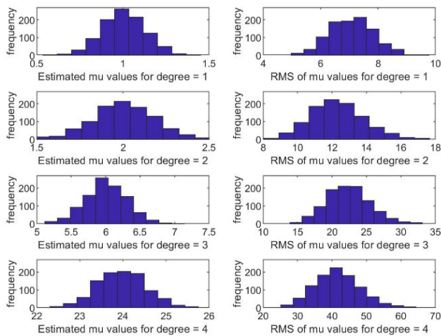
FIGURE 10. The left column shows the histograms of 1000 values of \langle \mu \rangle for degrees ranging from 1 to 4. The right column shows the histograms of 1000 values of \sigma_{\mu(q)} for degrees ranging from 1 to 4.
