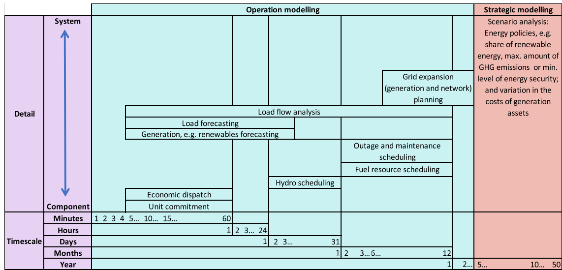
Fig. 3. Time horizon and electrical power system analysis.
