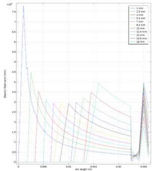
Figure 11. Electric field norm at Z=0 for different HV electrode radius, 30 cm length ground electrode
