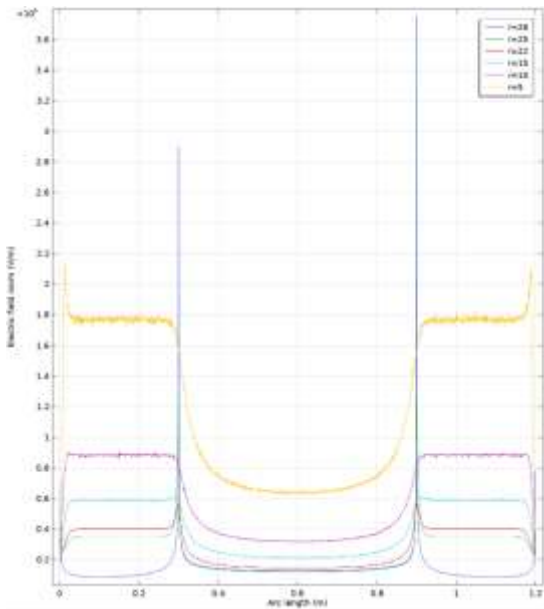
Figure 10. Electric field norm along vertical length of the reactor with ground electrode at both ends of the reactor
