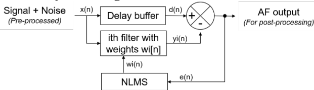
Fig. 4. Simplified block diagram of the AF algorithm implemented in the DDNR.
