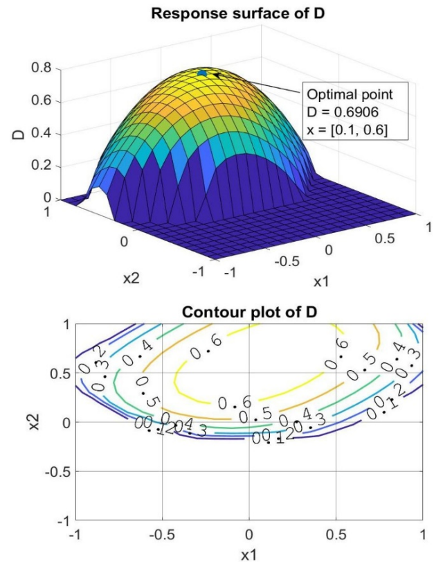
Fig. 8. Response surface and contour plot of overall desirability D with x3 and x4 set at 0.6 and -1 respectively.
