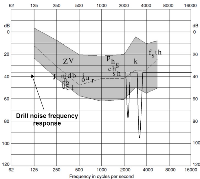
Fig. 2. ‘Speech banana’ frequency audiogram superimposed with a simplified frequency profile of an electric motor driven dental drill at no load (Adapted from Klingpornkun et.al [6])
