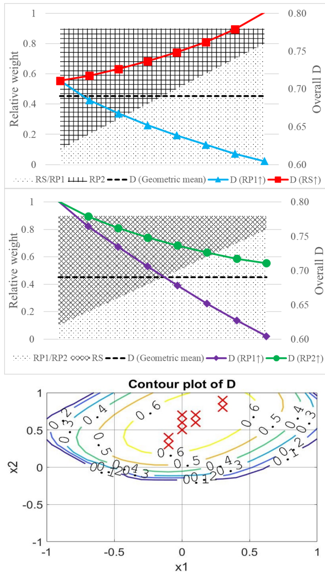
Fig. 11. Sensitivity analysis of overall desirability D with regard to different relative weights assigned to the three responses. In (a) and (b) varying responses are represented using different patterns. Overall D prediction using geometric mean is indicated by a horizontal black dotted line. In (c) all optimal points identified are depicted by red crosses.
