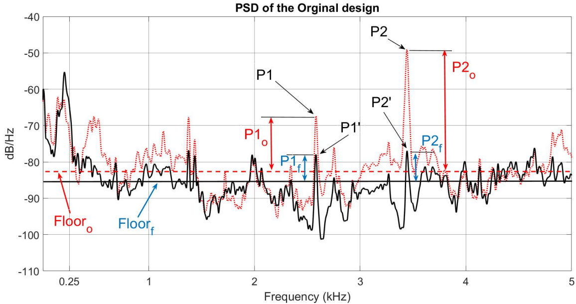
Fig. 5. Example PSD plot for the original design, i.e. nominal setting. The original signal is shown in red dotted line, the filtered signal is shown in black solid line. Signal floor values are shown by horizontal lines.
