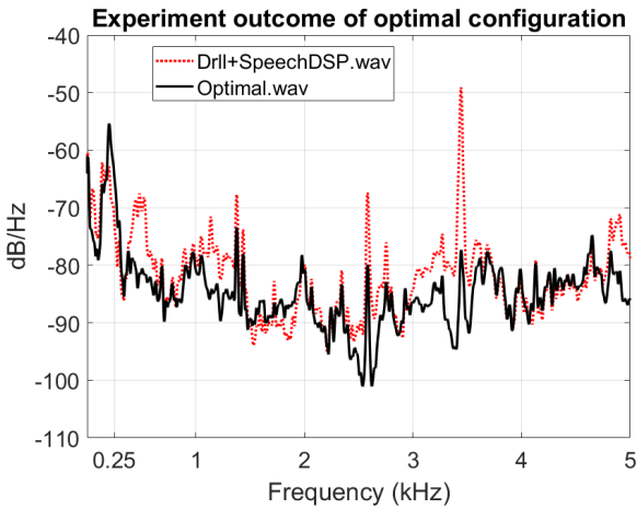
Fig. 9. PSD plot for the optimal design. The original signal is shown in dotted line, the optimised filtered signal is shown in solid line.
