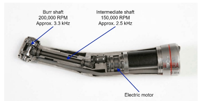
Fig. 1. Illustration of a typical electric dental drill (Adapted from Long Star Handpiece [4])
