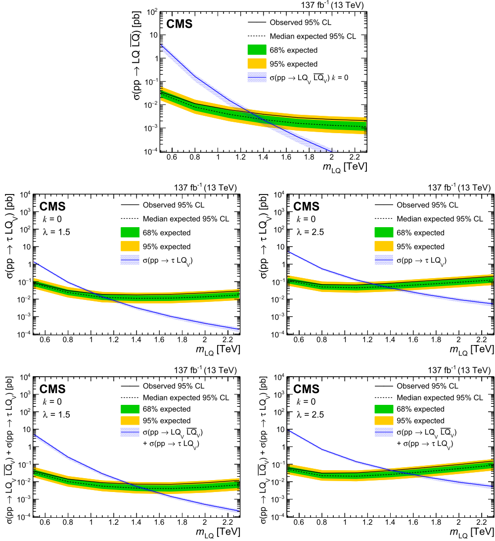
Fig. 4. The observed and expected (solid and dotted black lines) 95% CL upper limits on \sigma(pp \rightarrow LQ_V \overline{LQ}_V) (upper), \sigma(pp \rightarrow \tau LQ_V) with \lambda = 1.5 and 2.5 (middle left and right), and \sigma(pp \rightarrow LQ_V \overline{LQ}_V) + \sigma(pp \rightarrow \tau LQ_V) with \lambda = 1.5 and 2.5 (lower left and right), as a function of the mass of the LQ_V , with k = 0 . The limits apply under the assumption of equal couplings for the LQ decay to each of the two allowed lepton flavor pairings. The bands represent the one- and two-standard deviation variations of the expected limit. The solid blue curve indicates the theoretical predictions at LO.
