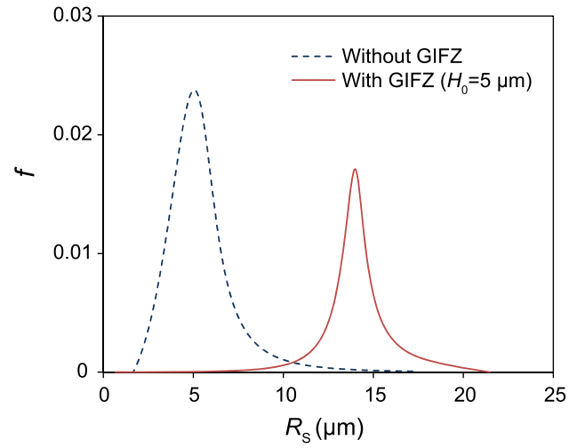
Fig. 5—Calculated size distribution of solid particles at recalescence ( R_s ) with and without consideration of GIFZ for Al-1Cu alloy with N_0 = 10^{13} \text{ m}^{-3} and \dot{T} = 3.5 \text{ K/s} .
