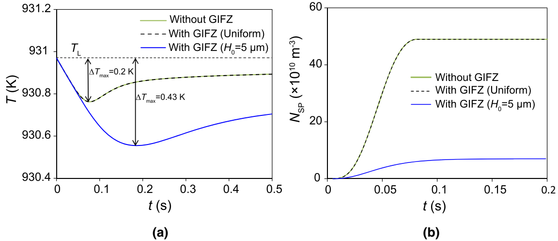
Fig. 4—Calculated (a) cooling curves and (b) the total number density of solid particles ( N_{SP} ) with and without consideration of GIFZ for Al-1Cu alloy with N_0 = 10^{13} \text{ m}^{-3} and \dot{T} = 3.5 \text{ K/s} (Color figure online).
