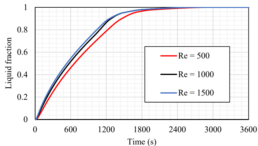
Figure 15. The liquid fraction development for the total PCM for case 3b ( T_{in} equals 50 °C) at different values of Re (500, 1000, and 1500).
