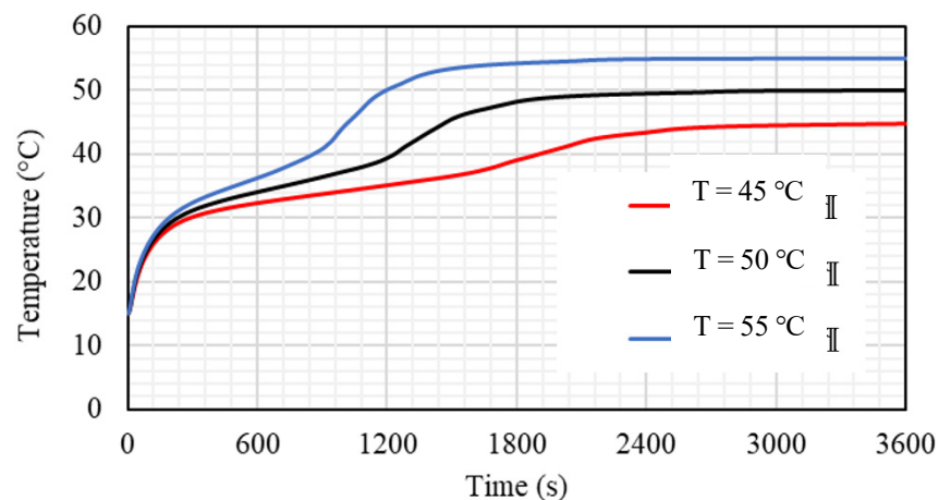
Figure 18. The average temperature of the PCM for the case 3b (Re equals 1000) at different values of inlet HTF temperature ( T_{in} = 45\text{ }^{\circ}\text{C} , T_{in} = 50\text{ }^{\circ}\text{C} , and T_{in} = 55\text{ }^{\circ}\text{C} ).
