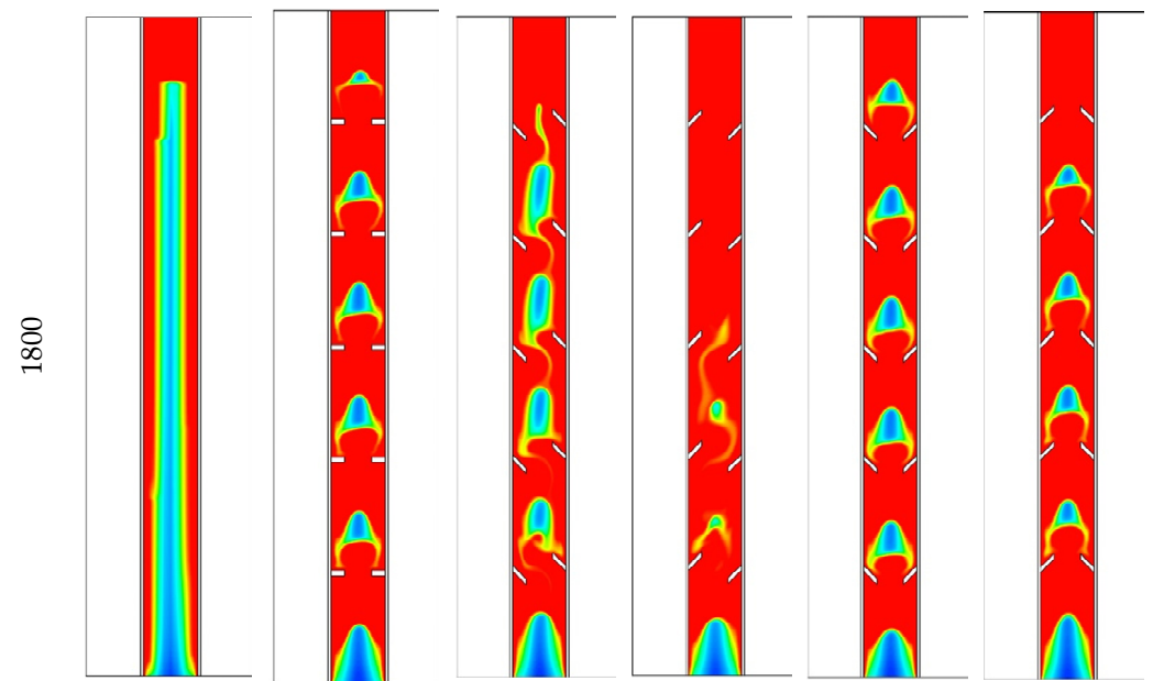
Figure 6. The liquid fraction development during 1800 s in three different time steps for the case of finless and the cases of different orientations of fins directions. Note that the right- and left-hand-side walls are the outer and the inner walls, respectively.
