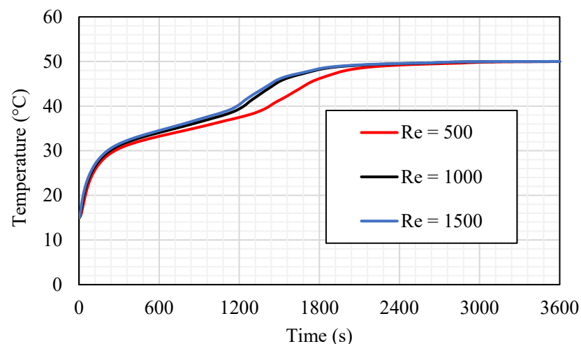
Figure 16. The average temperature profile for the total PCM for the case of 3b ( T_{in} equals 50 °C) at different values of Re (500, 1000, and 1500).
